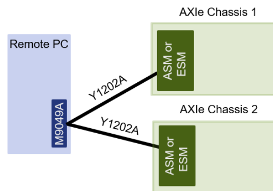
Figure 12. The M9049A can also be used for mid-performance (x8) connections from a remote PC to two AXle Chassis. PXle and AXle chassis can also be combined. Cable and chassis link depends on chassis capability (up to Gen 3).
