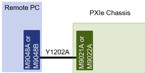
Figure 8. Use the M9048A with the M9021A in the M9018B (x8 Gen 2) or M9048B with the M9022A in all PXle chassis (x8 Gen 3 cable link). Chassis link depends on chassis capability
