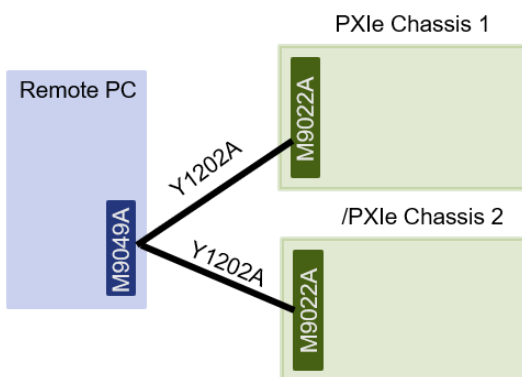
Figure 11. Use the M9049A for mid-performance (x8) connections from a remote PC to two PXle Chassis. Cable and chassis link depends on chassis capability (up to Gen 3).
