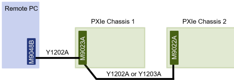
Figure 13. Combine the M9048B, M9022A, and M9023A for mid-performance (x8) connections from a remote PC for multiple PXle chassis (up to a total of four), depending on PC capability. Cable link is Gen 3, chassis link depends on chassis capability (up to Gen 3).
