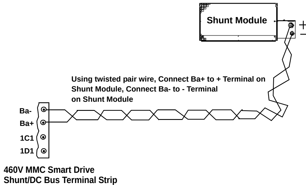
Figure 7-4: Wiring 460V MMC Smart Drive to 2800 Watt, 25 \Omega Shunt Module / 3900 Watt, 18 \Omega Shunt Module
