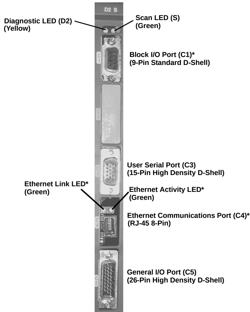
Figure 10-1: The Drive Resident Digital MMC Control
