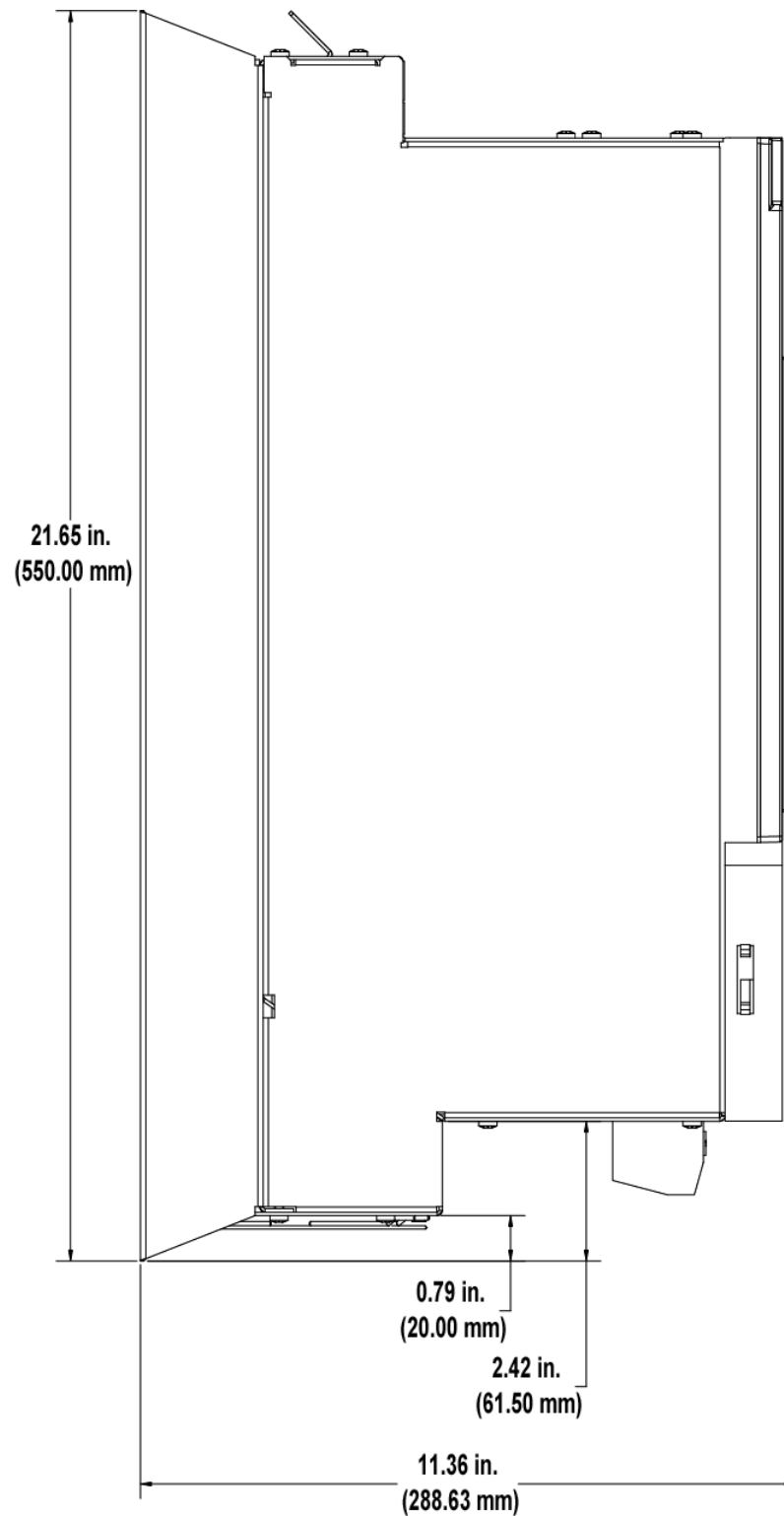
Figure 6-15: Size 3 460V Smart Drive - Side View
