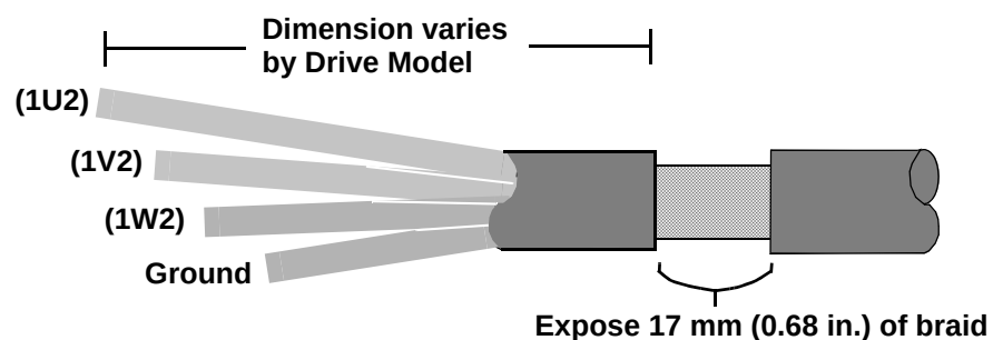
Figure 3-3: : Motor Cable
