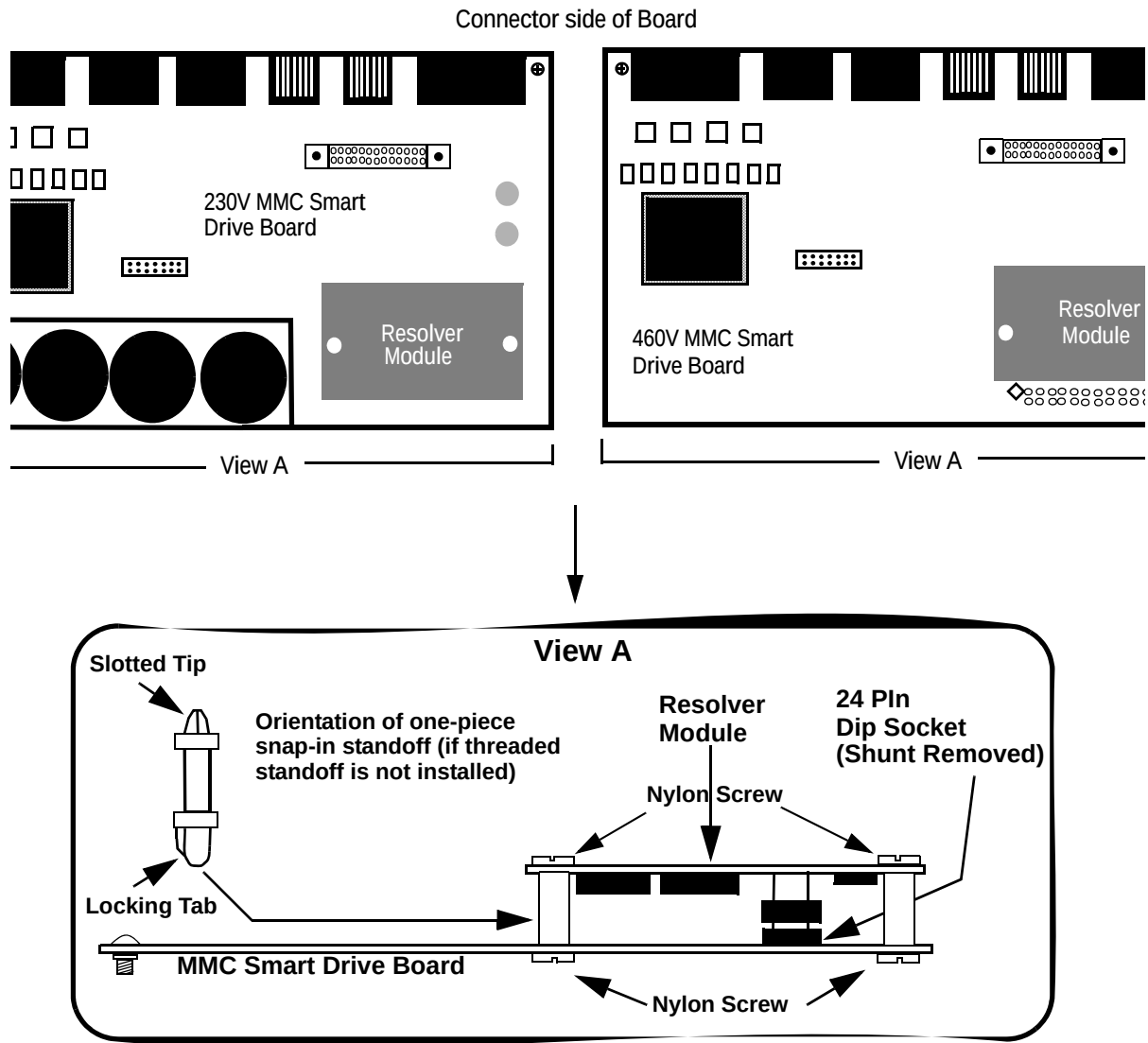
Figure 9-2: : Shunt Removed and Resolver Module Installed
