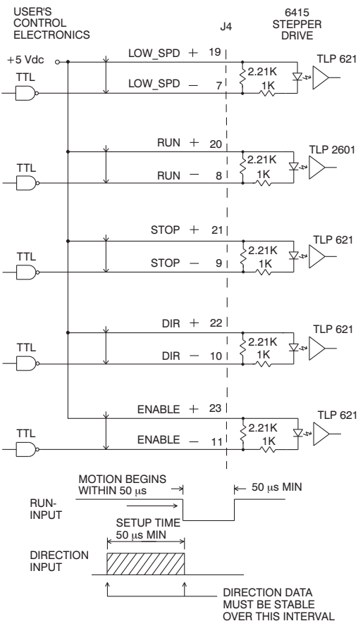
Figure C-8. Interface Circuits
