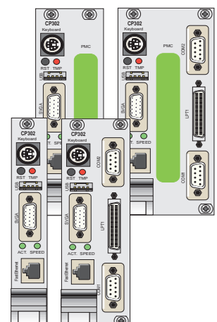
➤ CP302 - Front Panel
