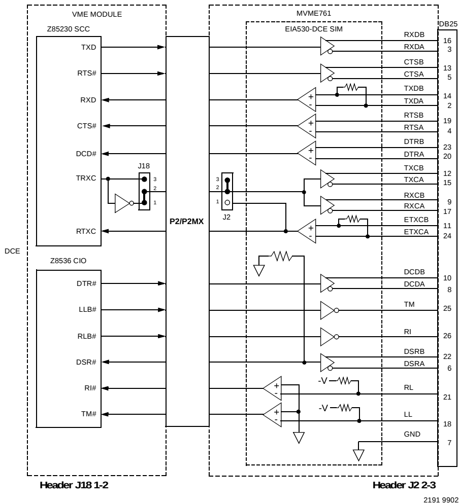
Figure 2-17. MVME761 EIA-530-DCE Configuration Port 3
