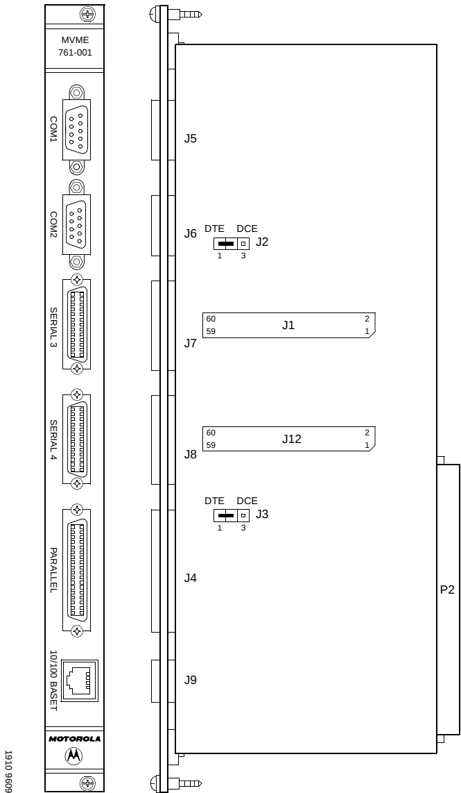
Figure 2-11. MVME761 Connector and Header Locations
