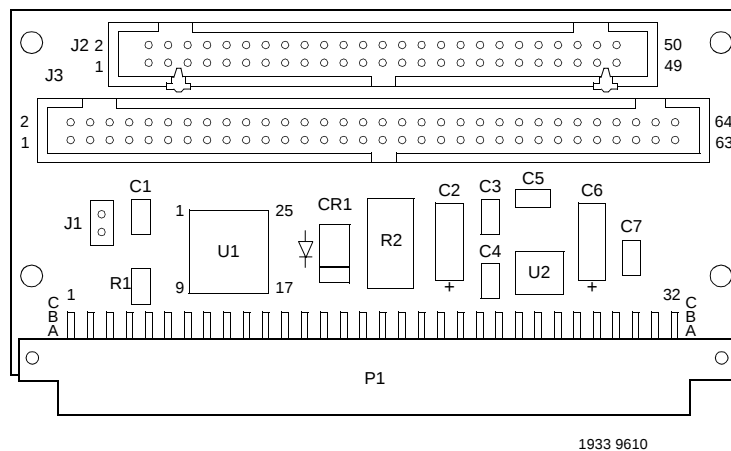
Figure 2-29. MVME761 Three-Row P2 Adapter
