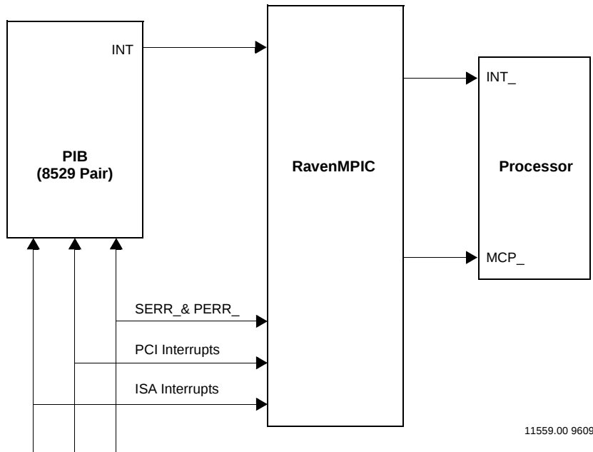
Figure 4-3. MVME2700 Interrupt Architecture
