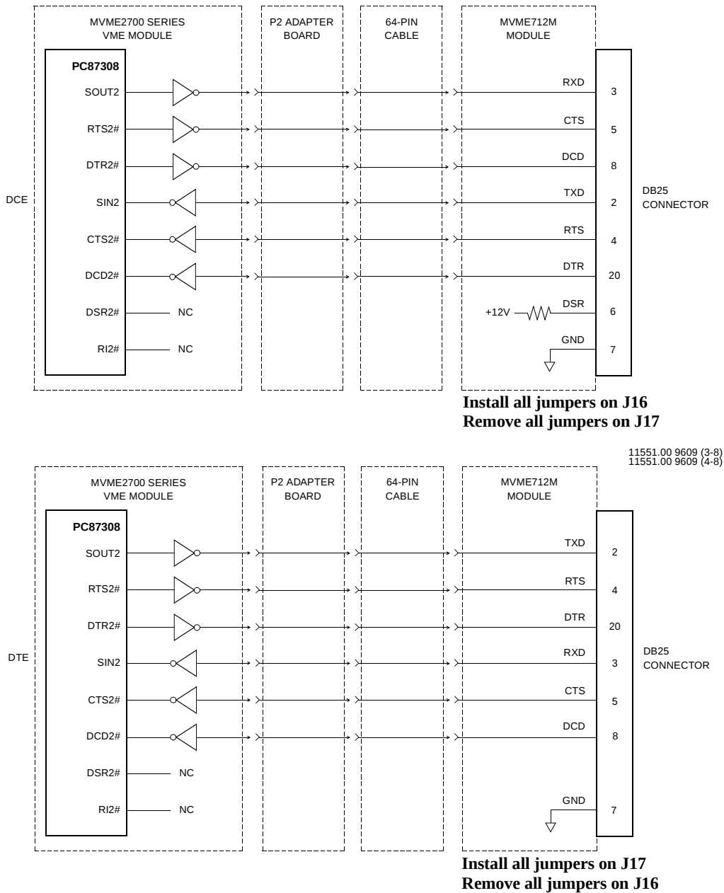
Figure 2-5. MVME712M Serial Port 2 DCE/DTE Configuration
