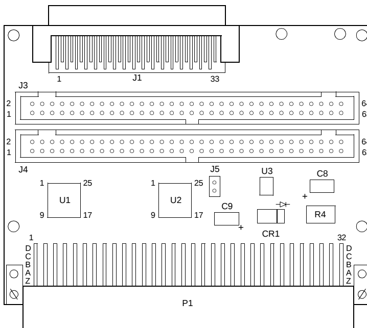
Figure 2-19. MVME761 Five-Row P2 Adapter
