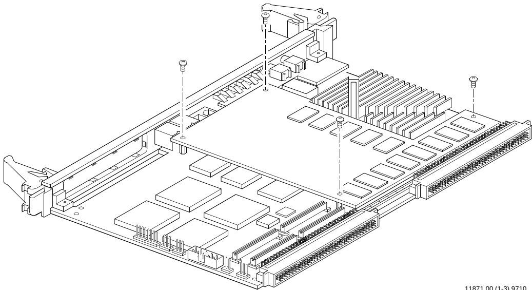
Figure 3-1. RAM200 Placement on MVME2700
