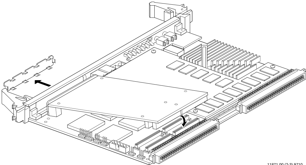
Figure 3-2. PMC Module Placement on MVME2700
