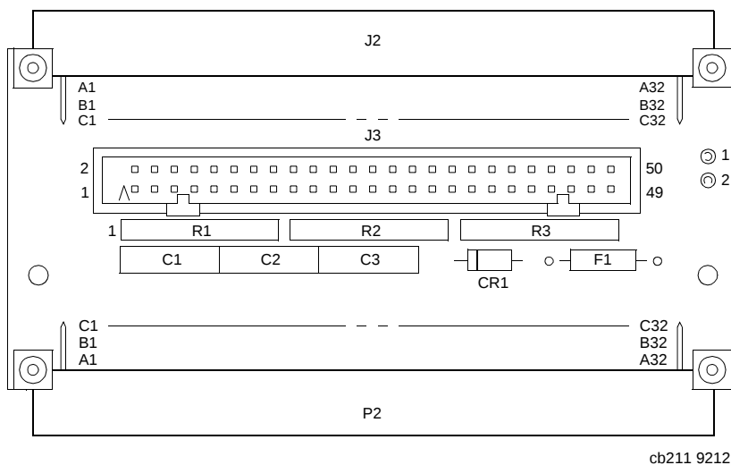
Figure 2-10. MVME712M Three-Row P2 Adapter
