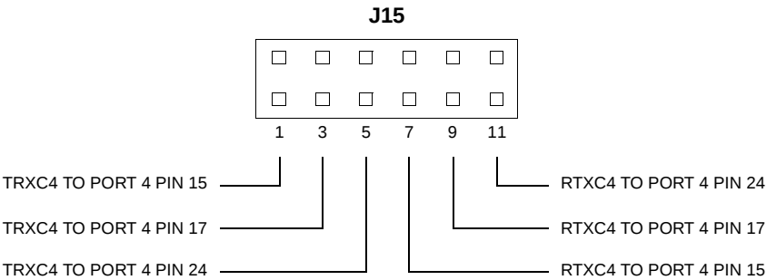
Figure 2-3. J15 Clock Line Configuration
