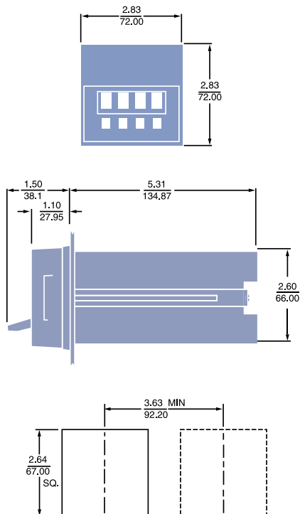
PANEL CUTOUT SHOWING DISTANCE BETWEEN ADJACENT CUTOUTS.
