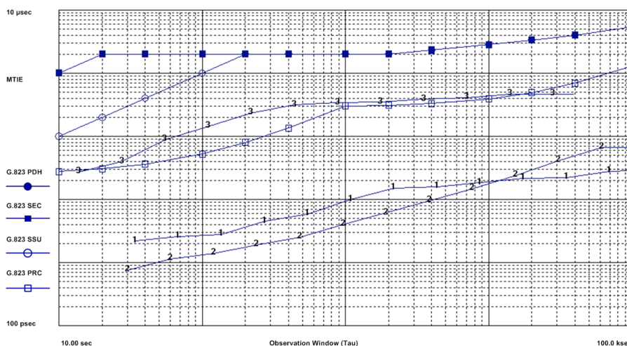
Figure 2. Three MTIE Measurements Compared to Four Telecom Masks
