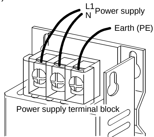
Terminal block diagram for noise filter connection
