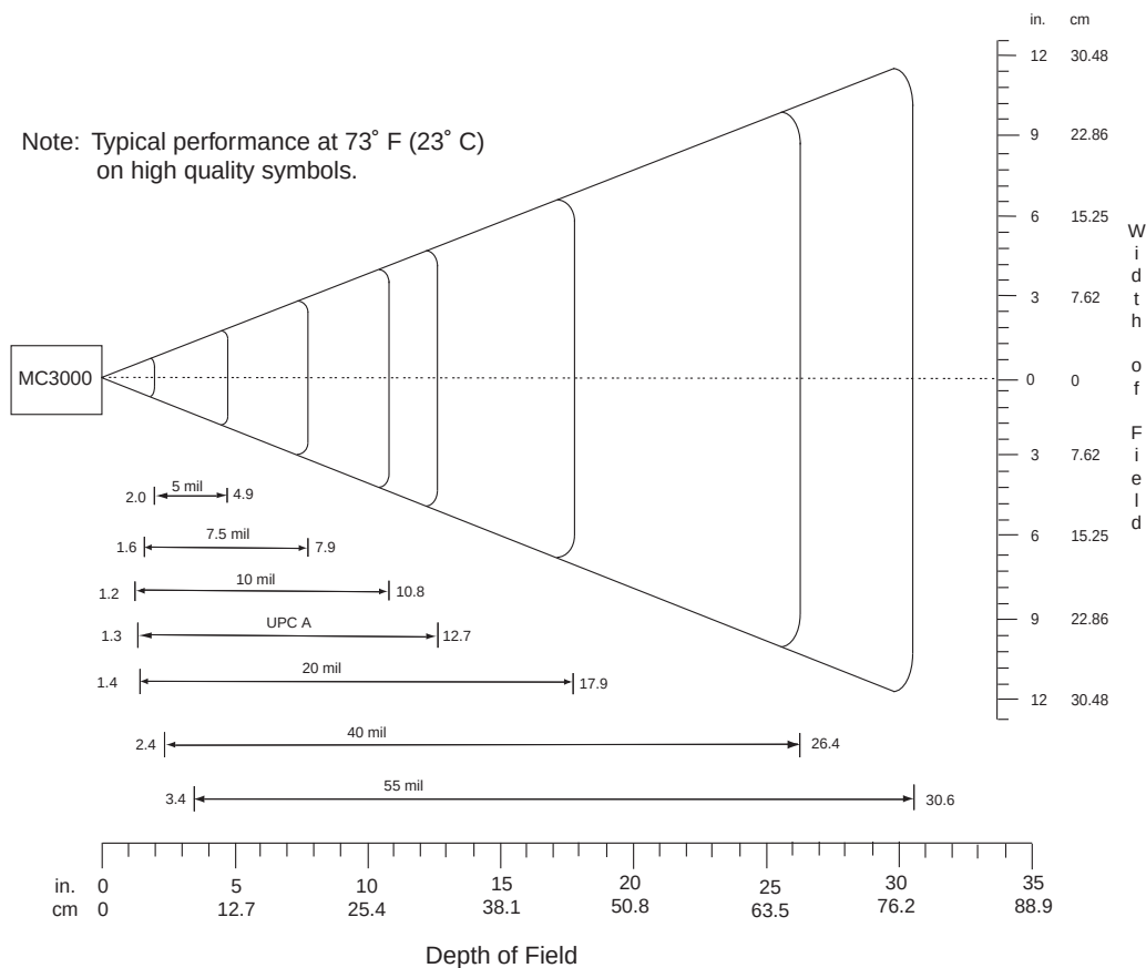
Figure 2-28 MC3000 Laser Decode Ranges
