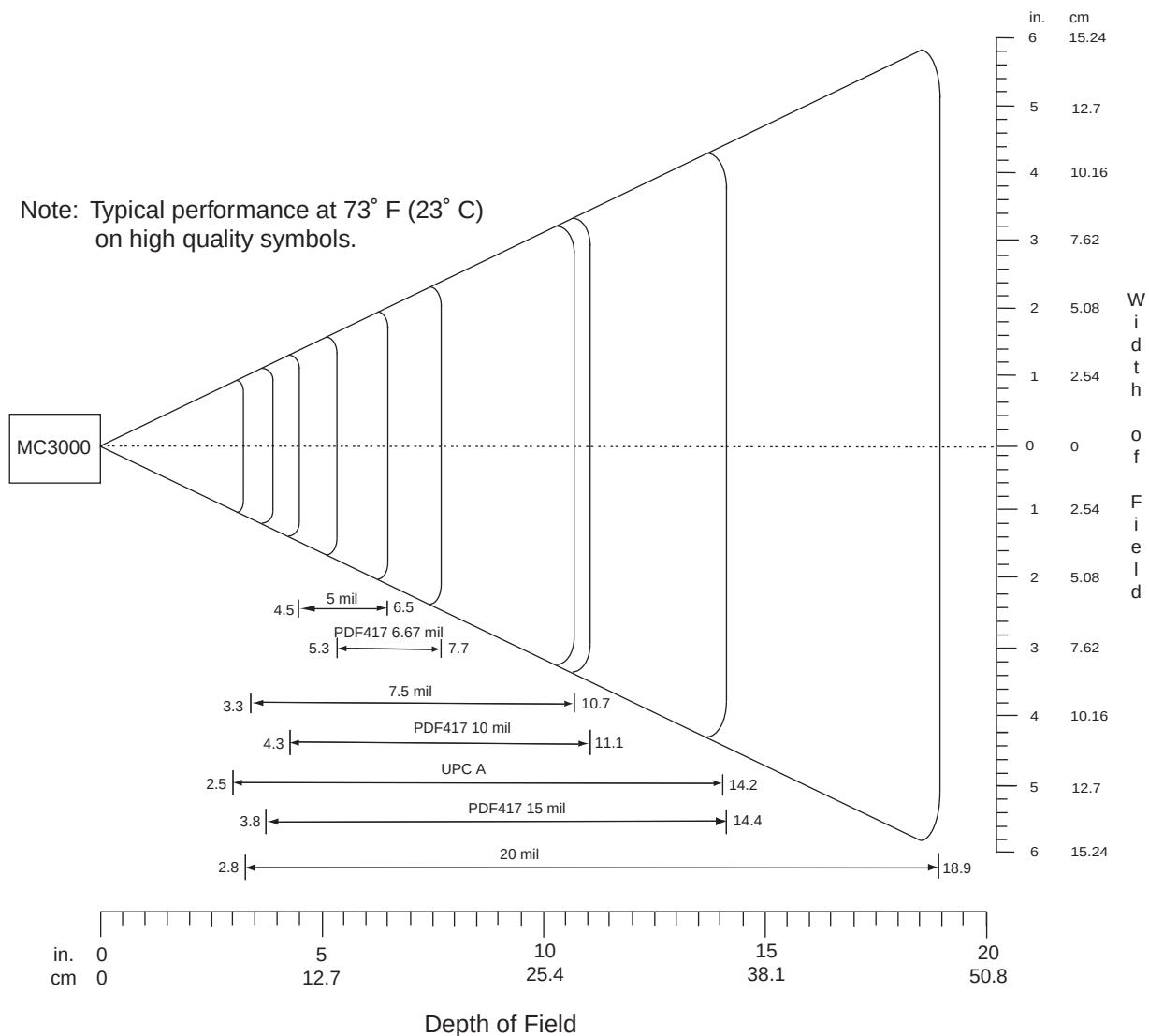
Figure 2-33 MC3000 Imager Decode Ranges
