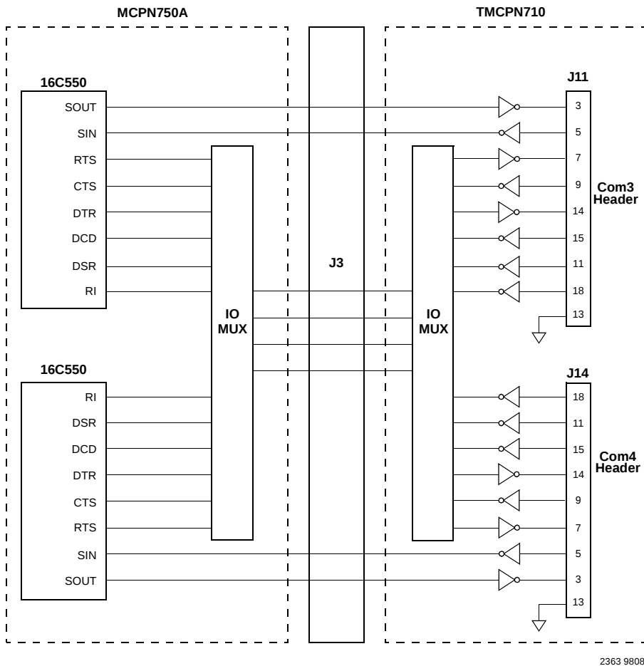
Figure 1-5. TMCPN710 Serial Ports 3 and 4
