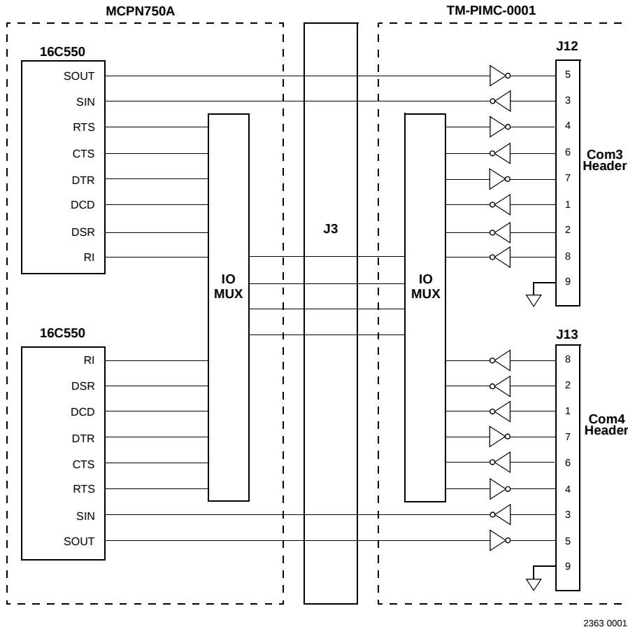
Figure 1-8. TM-PIMC-0001 Serial Ports 3 and 4
