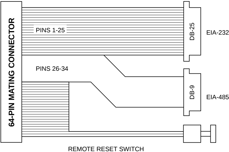
Figure 2-3. Cabling Connections to P2, Suggestion 2
