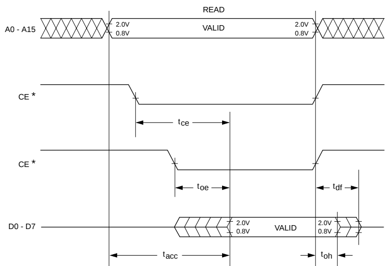
Figure 4-9. ROM/PROM/EPROM/EEPROM Read Timings Required by MVME133XTS
