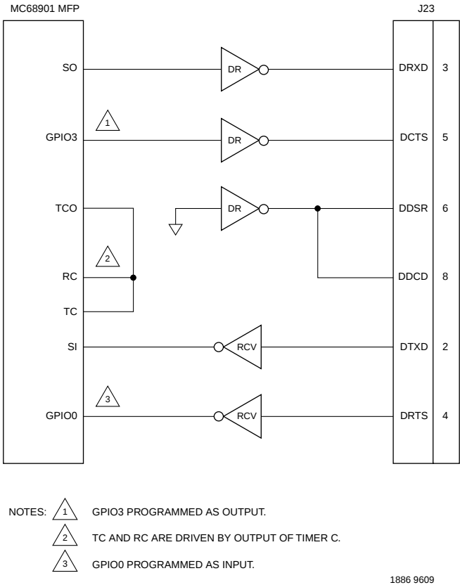
Figure 4-3. MVME133XTS Debug Port (to Terminal Only)
