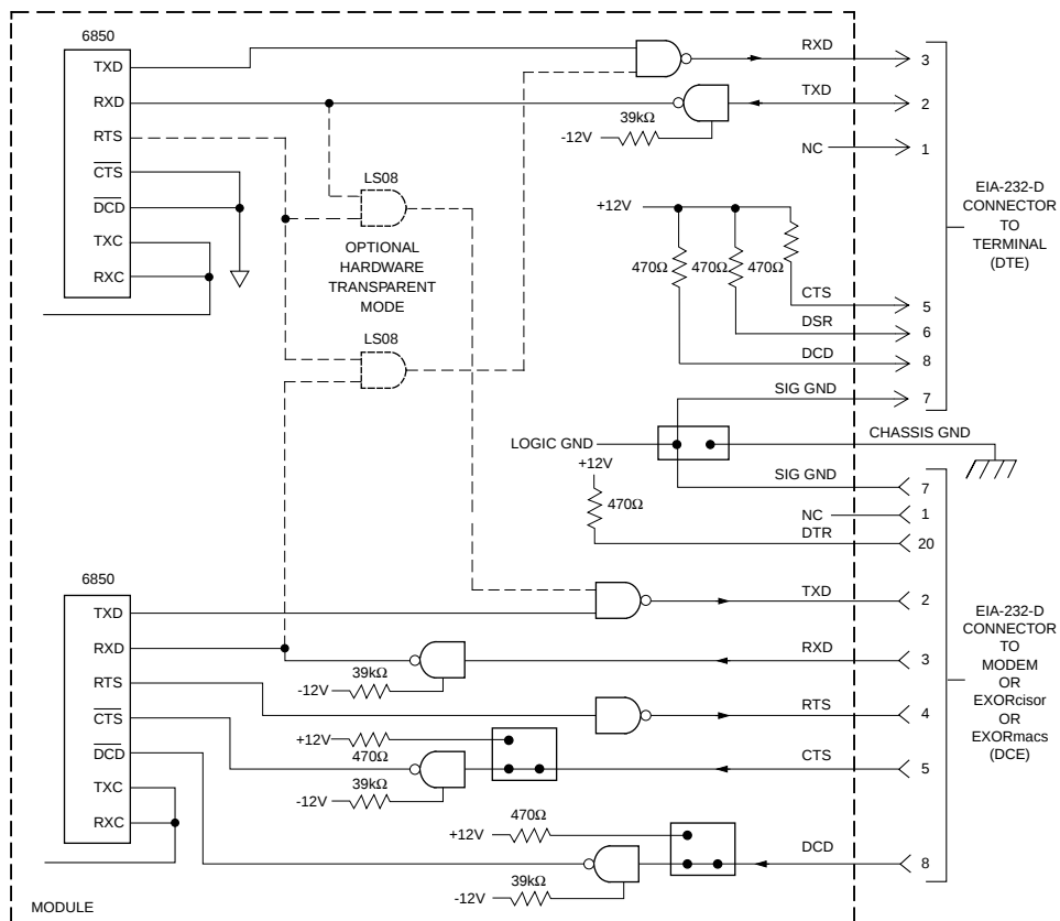
Figure B-1. Middle-of-the-Road EIA-232-D Configuration
