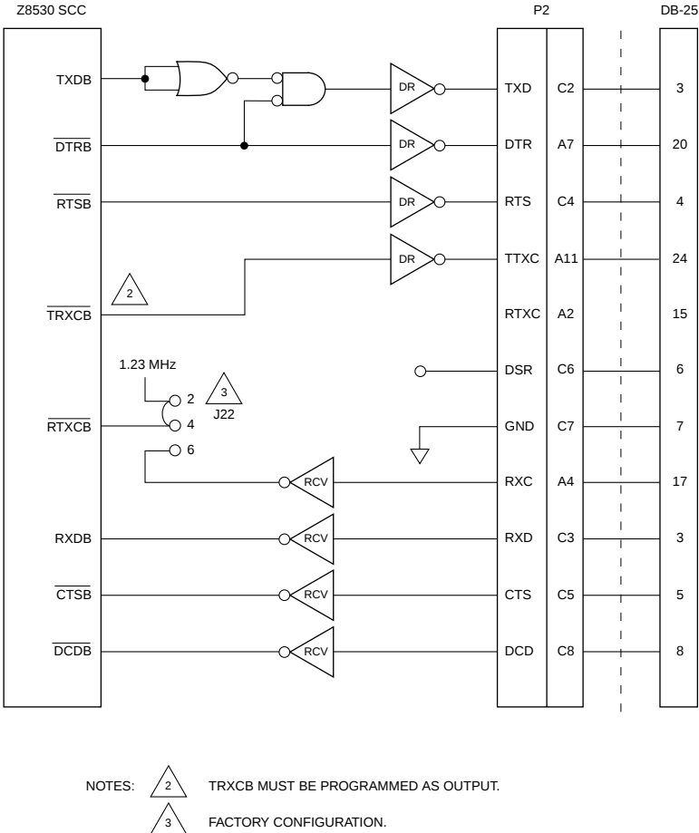
Figure 4-7. MVME133XTS EIA-232-D Port Configured as DTE (to Modem) with RTXCB Not Used
