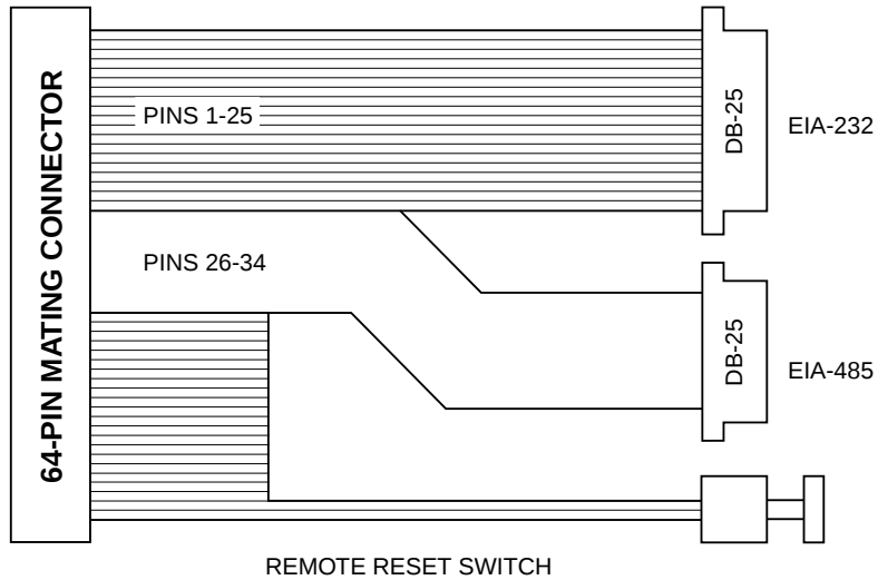
Figure 2-2. Cabling Connections to P2, Suggestion 1
