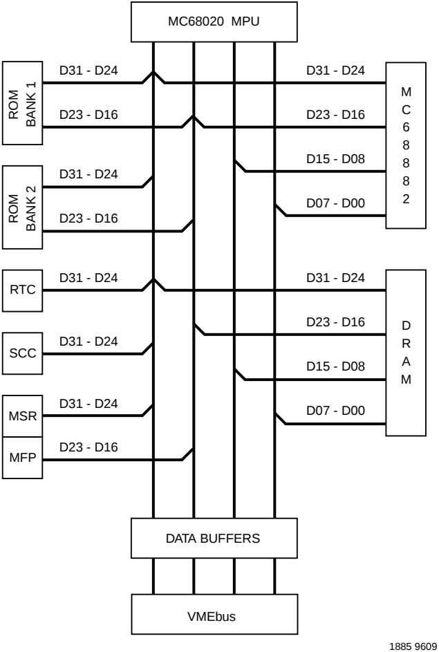
Figure 4-2. MVME133XTS Data Bus Structure
