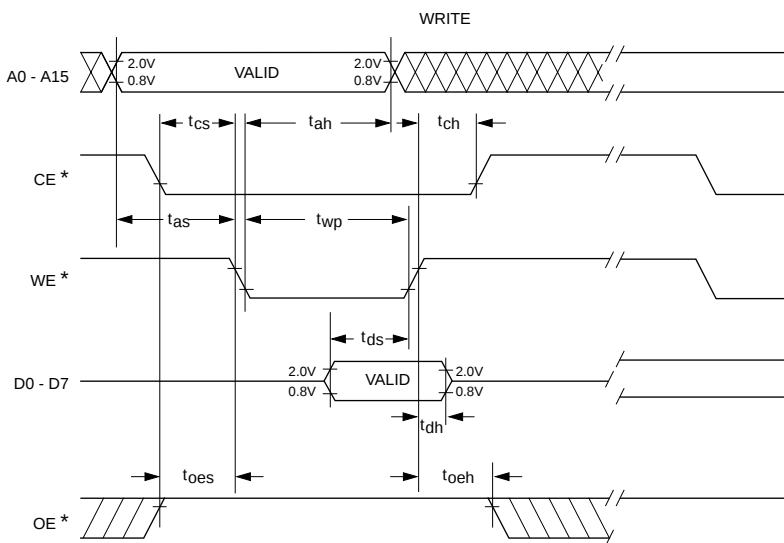
Figure 4-10. EEPROM Write Timings Guaranteed by MVME133XTS
