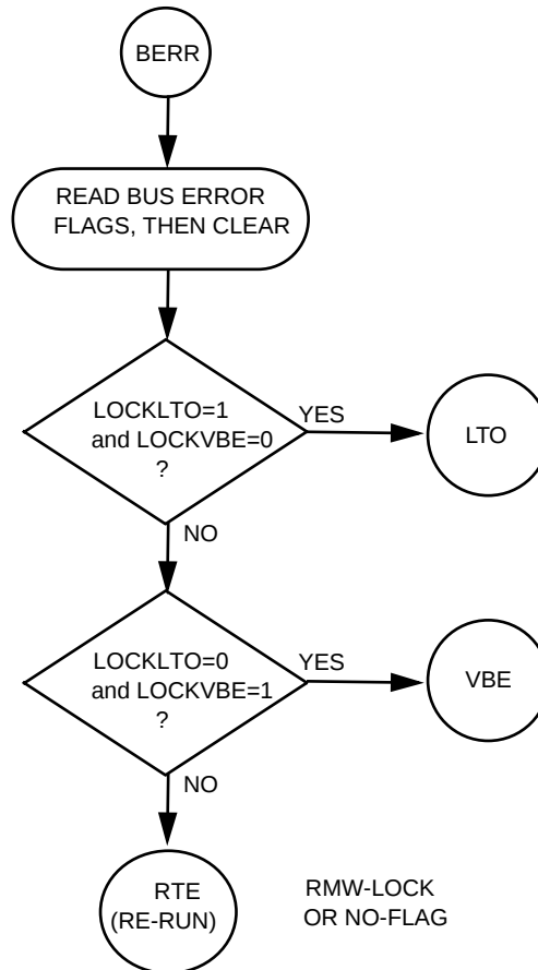
Figure E-1. Bus Error Exception Handler Flowchart for MVME133XTS
