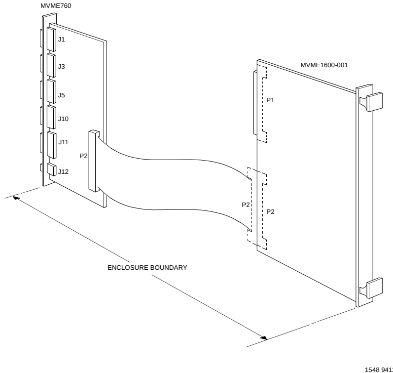
Figure 1-12. MVME760/MVME1600-001 Cable Connections
