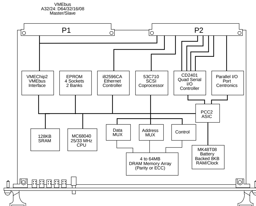
MVME167 block diagram
