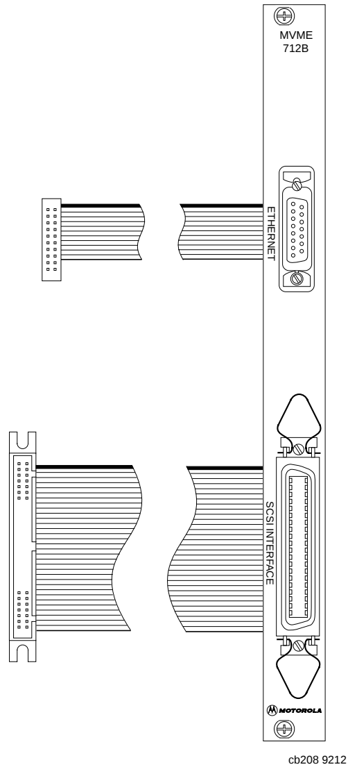
Figure 2-5. MVME712B Connector Locations
