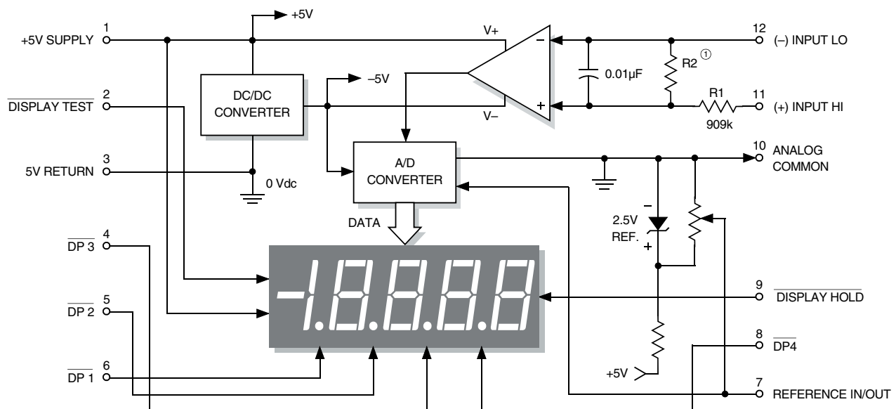
Figure 1. DMS-40PC Series Simplified Schematic
