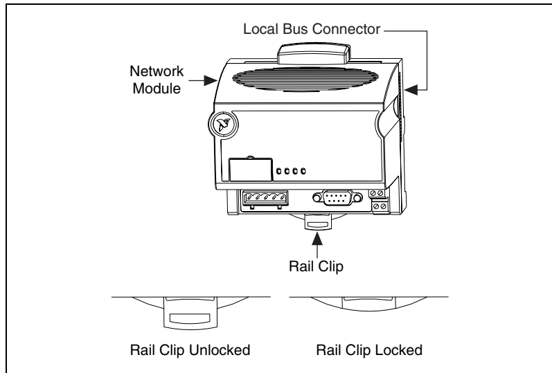
Figure 2-5. FieldPoint Network Module
