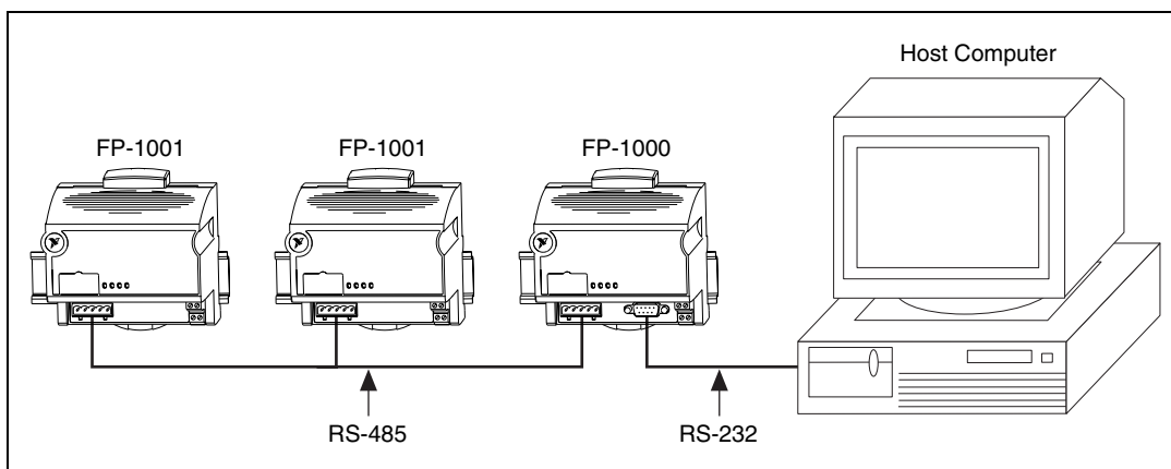
Figure 2-8. Host Computer Connected to One FP-1000 and Two FP-1001 Network Modules
