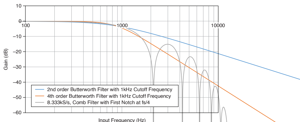
Figure 9. Comparing Magnitude Response of NI-9253 Filters
