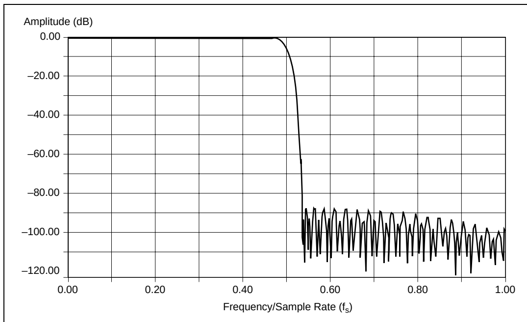
Figure 6-1. Input Frequency Response
