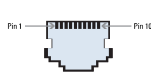
Figure 2. 10-Position Modular Jack Pin Locations
