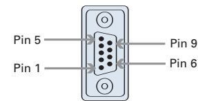
Figure 1. DB-9 Connector Pin Locations
