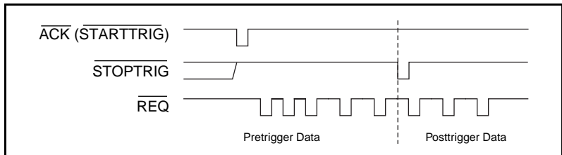
Figure 5-1. Pattern-Generation Timing
