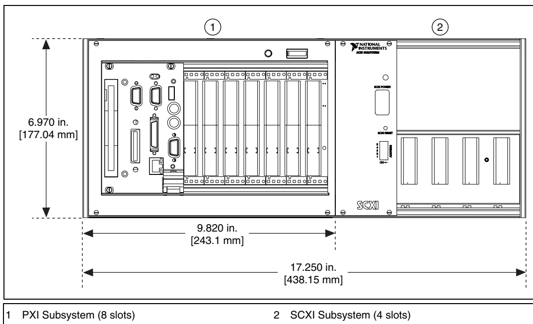
Figure A-1. PXI-1010 Dimensions (Front View Shown)
