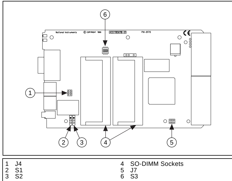
Figure 3-2. PXI-8170 Series CPU Board Parts Locator Diagram
