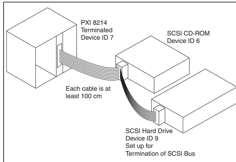
Figure 2-3. Multiple SCSI Devices with Termination Handled by the Last SCSI Device on the Bus
