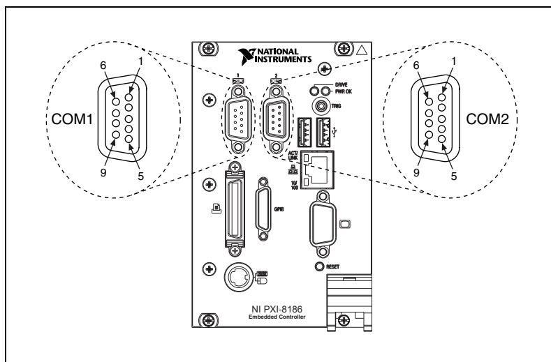
Figure 3-3. COM1 and COM2 Connector Location and Pinout
