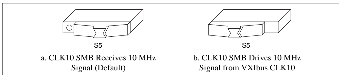
Figure 3-4. SMB CLK10 Direction
