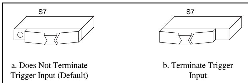
Figure 3-7. SMB Trigger Input Termination
