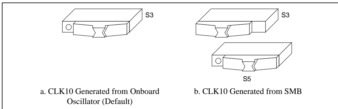
Figure 3-3. VXIbus CLK10 Routing
