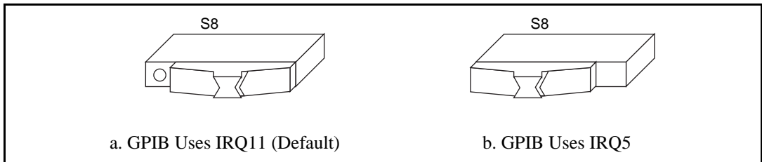
Figure 3-11. GPIO Interrupt Level
