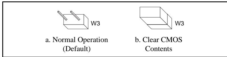
Figure 4-6. System CMOS
