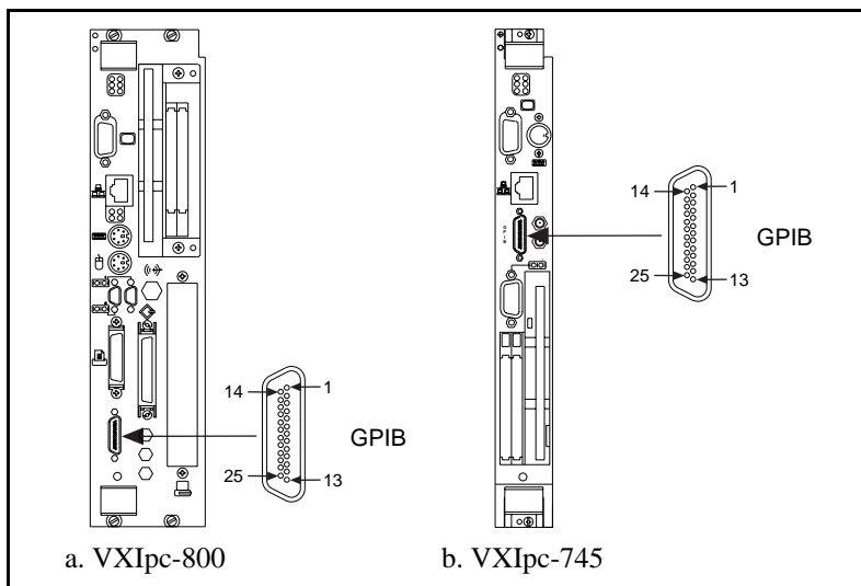
Figure E-10. GPIB Connector Location and Pinout
