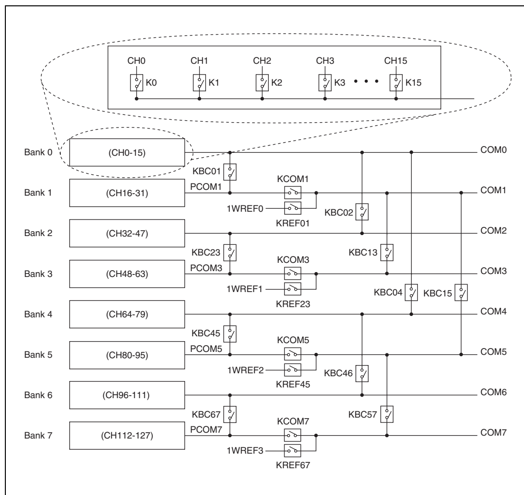
Figure 1. NI PXI-2530 Hardware Diagram (All Relays Open)
