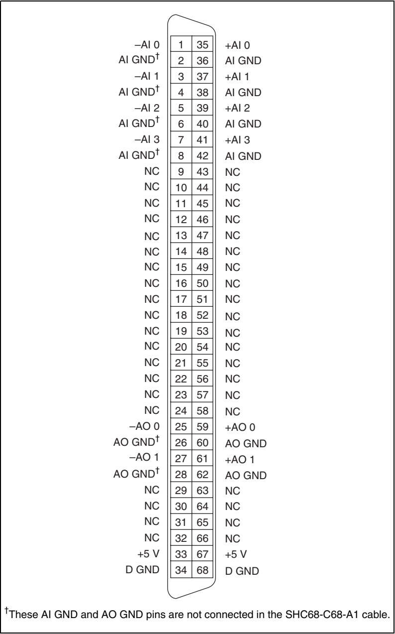
Figure 3-1. BNC-2140 External 68-Pin Analog Connector
