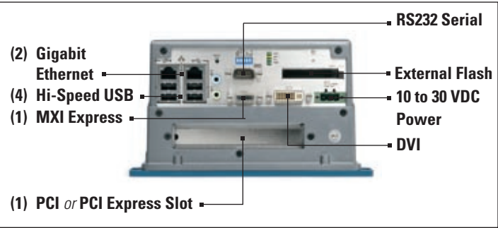
Figure 1. NI Industrial Controller Connectivity Options
