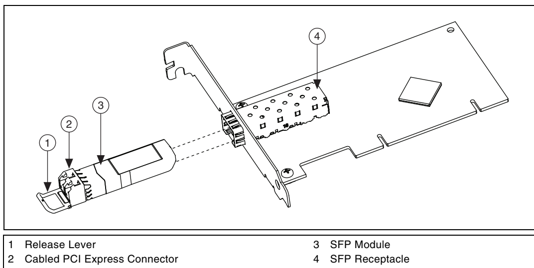
Figure D-1. SFP Module Removal
