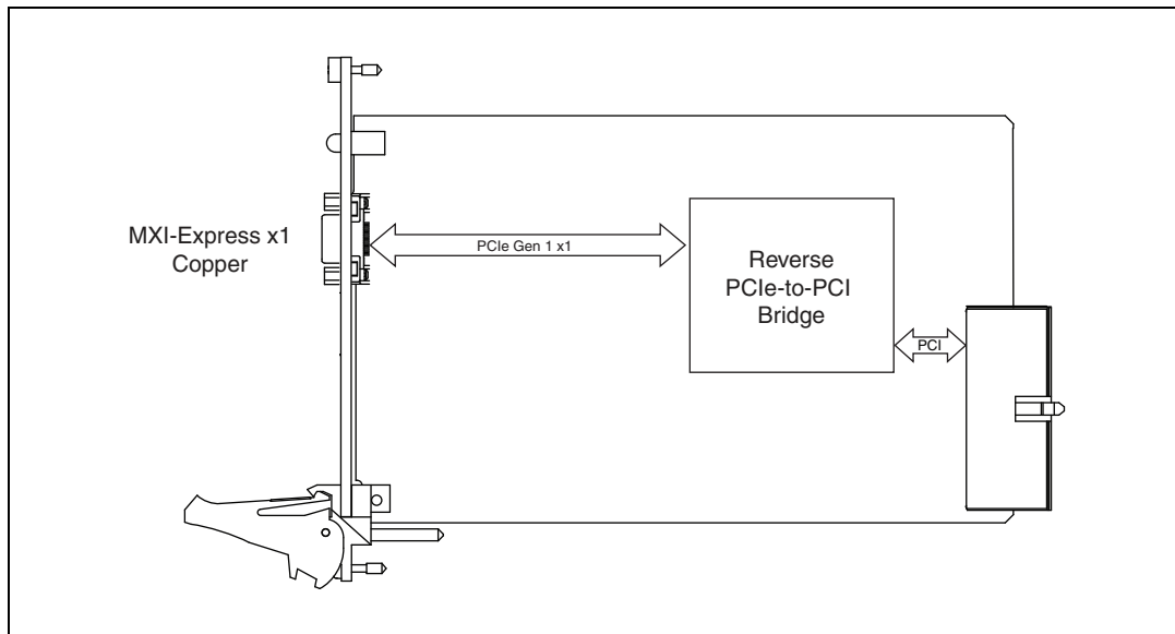
Figure 1-6. NI PXI-8364 (199991x-02L) Block Diagram
