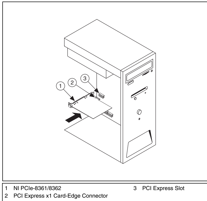
Figure 3-1. NI PCIe-8361/8362 Card Installation Example
