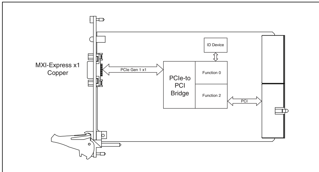
Figure 1-5. NI PXI-8360 (191373x-01) Block Diagram
