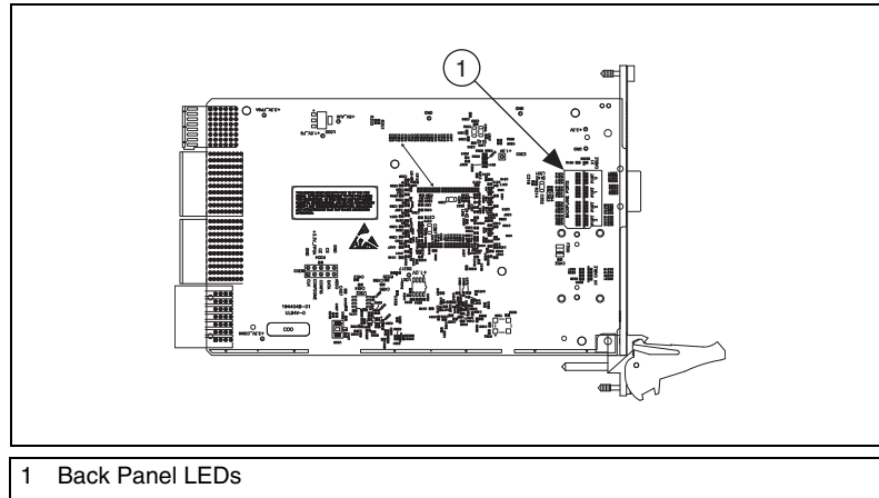
Figure 3-6. NI PXIe-8360 Back Side LED Locations
