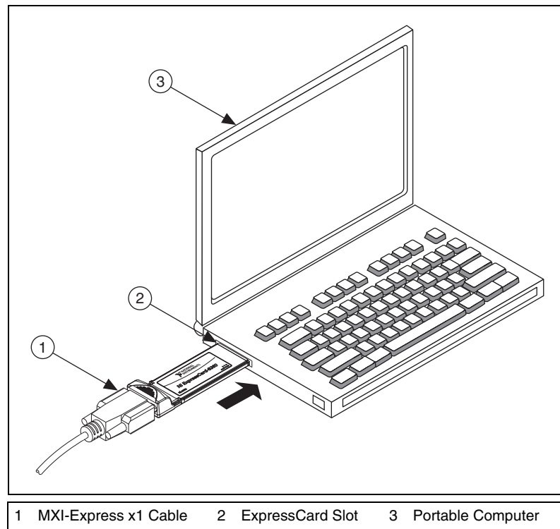
Figure 3-3. Installing the NI ExpressCard-8360 Into a Laptop
