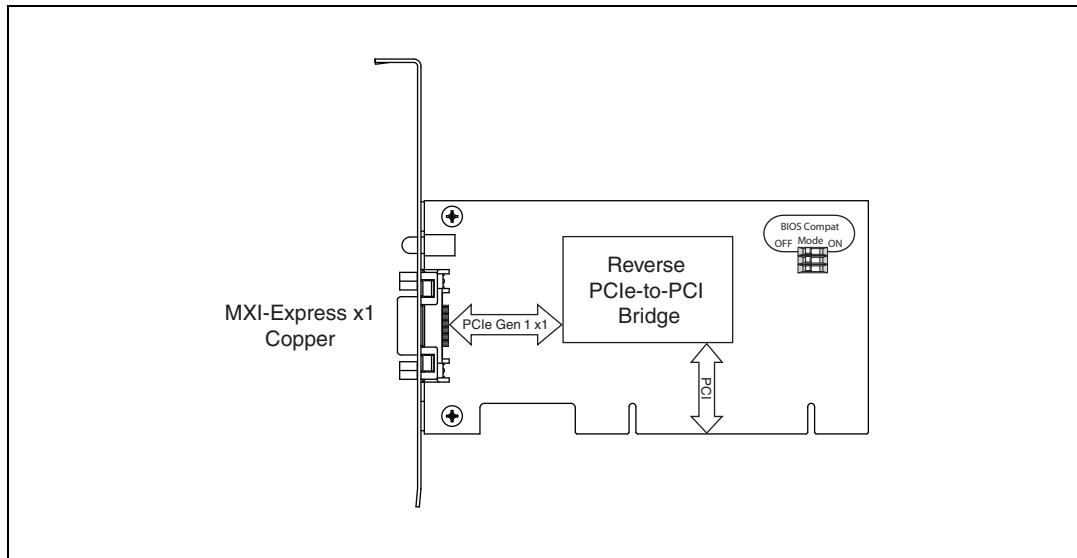
Figure 1-1. NI PCI-8361 (199392x-01L) Block Diagram
