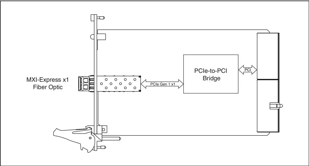
Figure C-3. NI PXI-8366 (199991x-03L) Block Diagram
