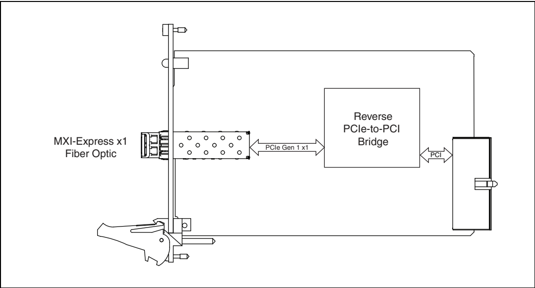
Figure C-4. NI PXI-8367 (199991x-04L) Block Diagram
