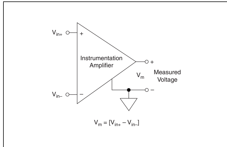
Figure 2-4. NI 783xR/784xR/785xR Instrumentation Amplifier
