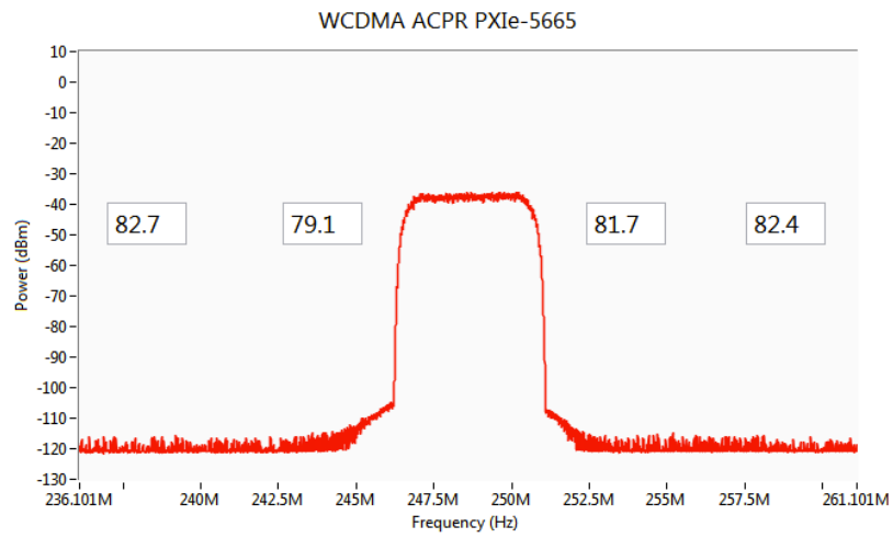
Figure 2. ACPR Measurement on a WCDMA (TM1 64 DPCHs) Signal Generated by a Vector Signal Generator Connected to a Filter
