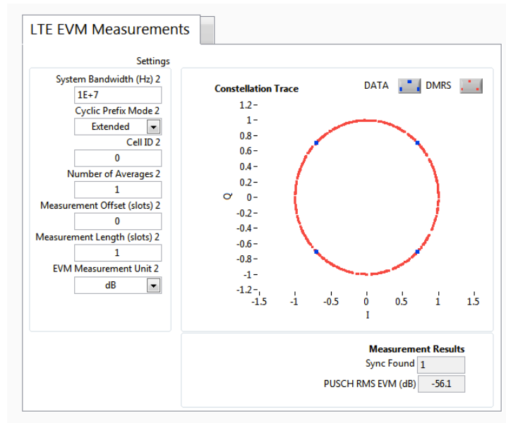
Figure 3. EVM Measurement of -56.1 dB on a LTE Signal Generated by an NI PXIe-5673
