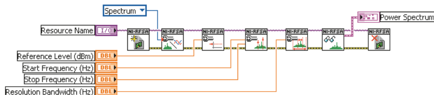
Figure 7. NI LabVIEW Example for Spectrum Sweep
