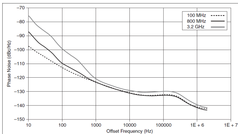
Figure 1. Phase Noise
