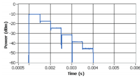
Figure 6. Deterministic 500 \mu s Power Steps Using the NI PXIe-5665 and RF List Mode
