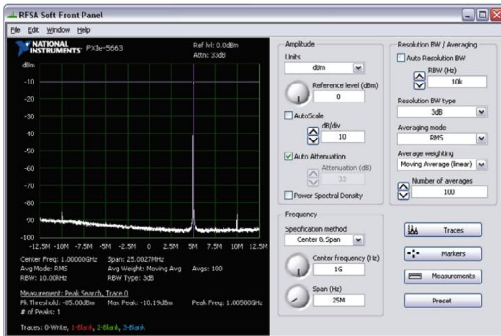
Figure 8. NI-RFSA Soft Front Panel
