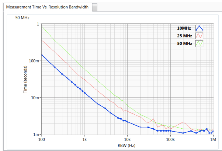
Figure 5. Measurement Time Versus Resolution Bandwidth for Spans of 10, 25, and 50 MHz
