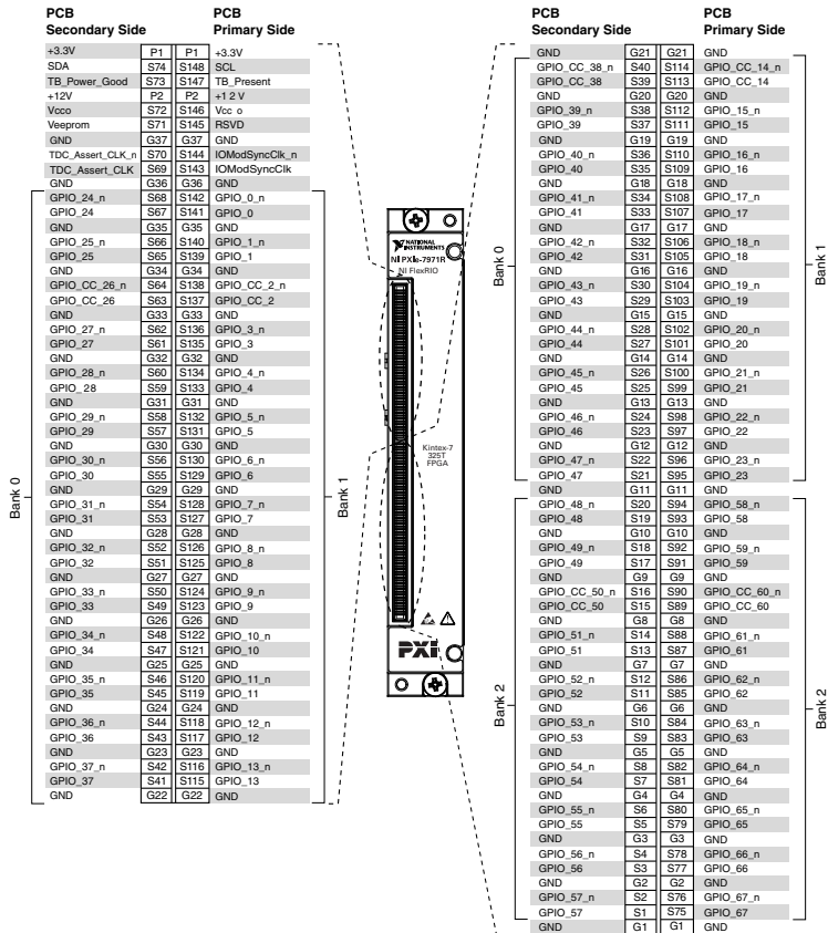
Figure 2. NI FlexRIO FPGA Module Front Connector Pin Assignments and Locations
