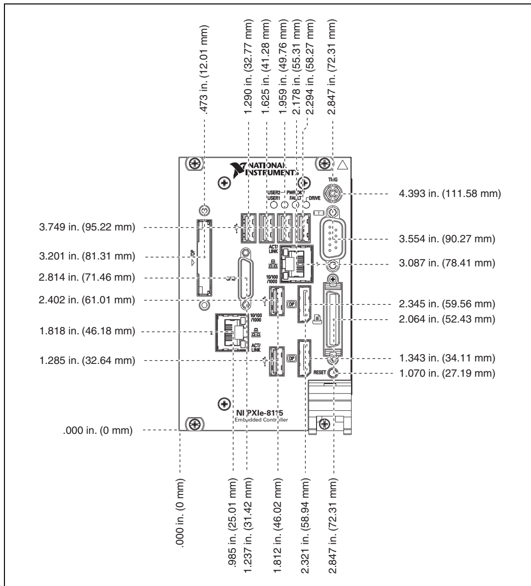
Figure 3-1. NI PXIe-8115 Front Panel Layout and Dimensions
