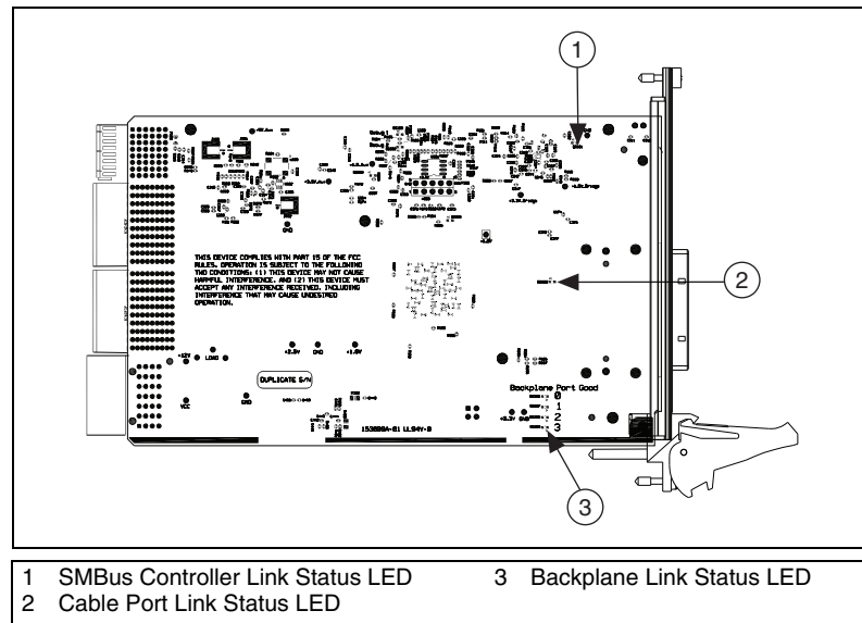
Figure 2-5. NI PXIe-8381 Back Side LED Locations
