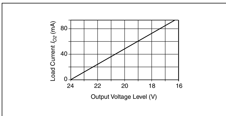
Figure 4. Load Current versus Output Voltage, Configuration 2
