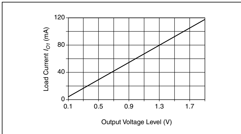
Figure 3. Load Current versus Output Voltage, Configuration 1
