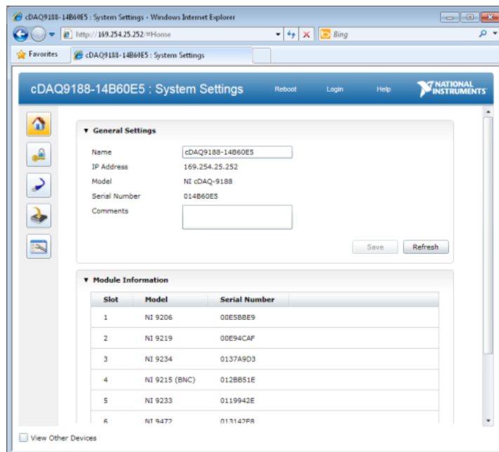
Figure 5. With the embedded web server on any Ethernet NI CompactDAQ chassis, you can remotely configure your NI CompactDAQ system from a web browser.
