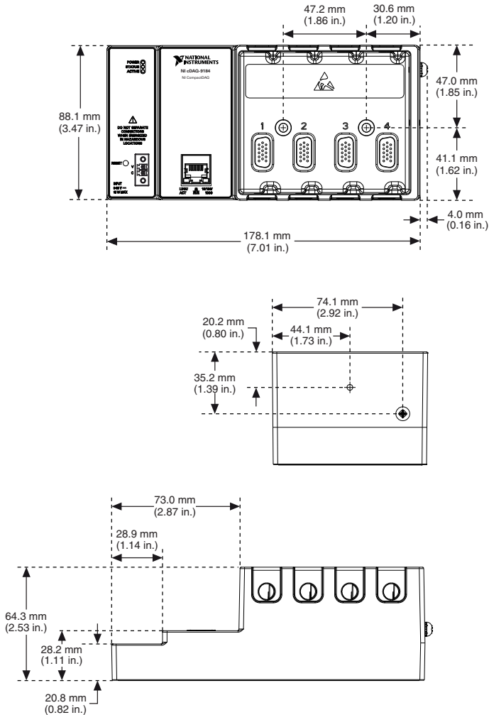
Figure 1. NI cDAQ-9184 Dimensions
