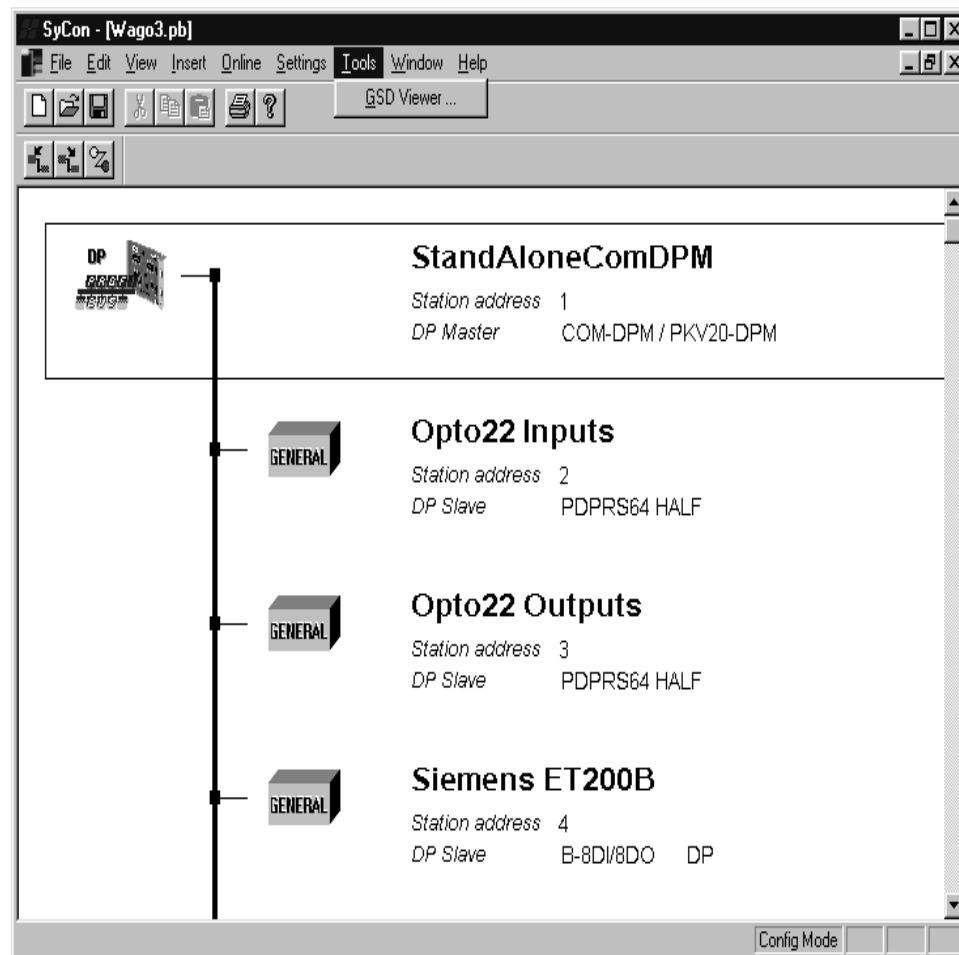
ProfiBus-DP Master
