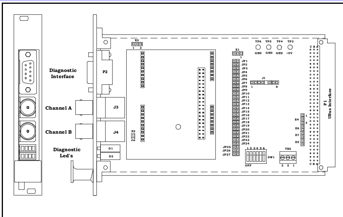
PMAC Gateway 3U ControlNet Version
