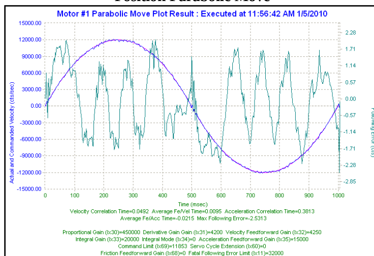
Position Parabolic Move
