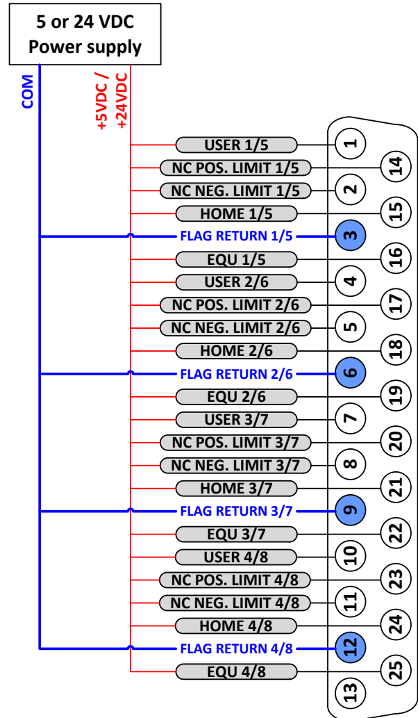
Sinking Limits And Flags
