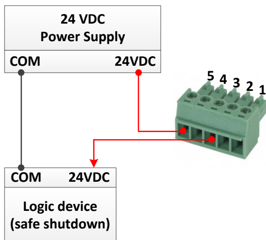
Watchdog Output, Normally Open
