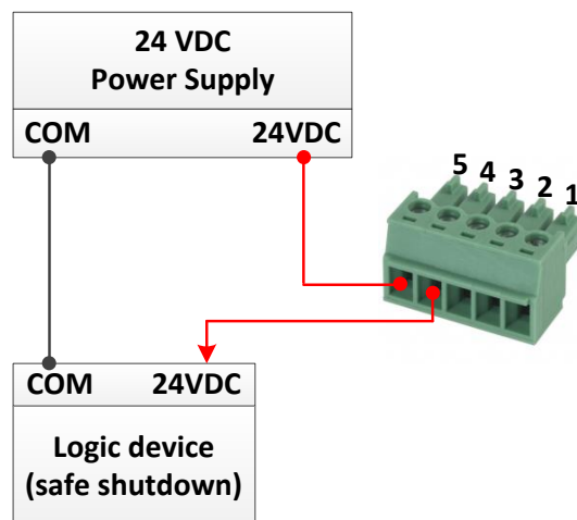
Watchdog Output, Normally Closed
