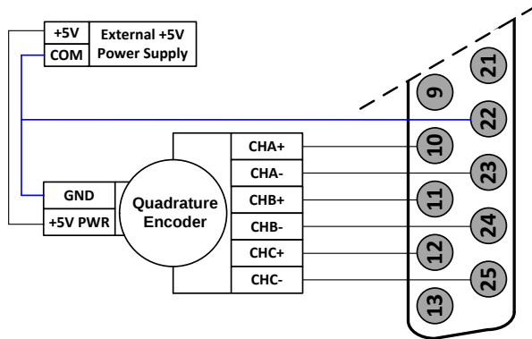
Differential Handwheel
