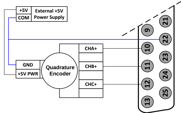
Single ended Handwheel
