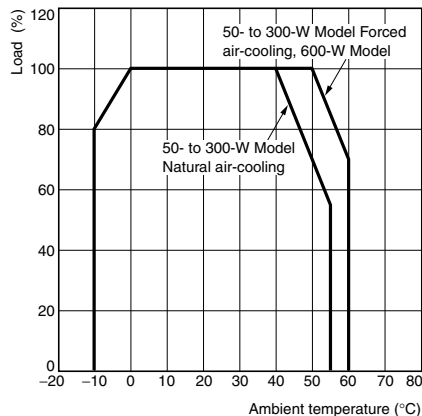
Covered Type
