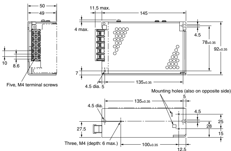
Mounting Holes
