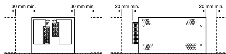
Standard Installation (600-W Model)
