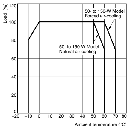
Standard Installation (50-W Model)
