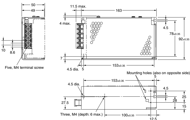
Mounting Holes
