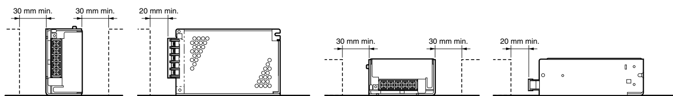
Standard Installation (300-W Model)
