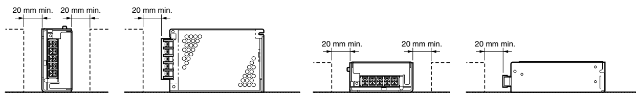
Standard Installation (100/150-W Model)
