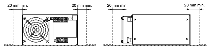
Standard Installation (600-W Model)
