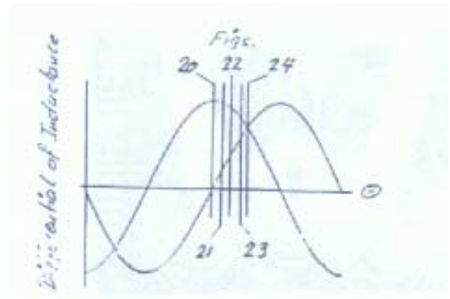
Figure 25. Inductance variation vs. position.
