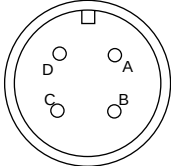
R20 Series Only MS3101A20-4P
