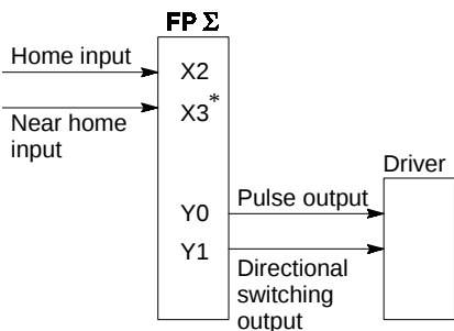
Figure 89: FPΣ Pulse output function - I/O allocation when using CH0 (single pulse input)
