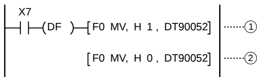
Figure 71: FPΣ Program of high-speed counter control instruction "F0"
