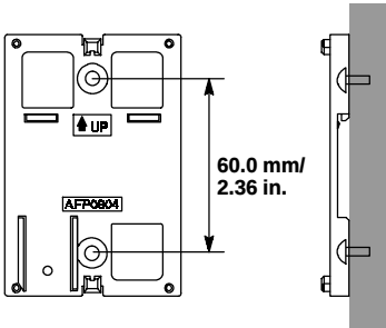
Figure 32: FPΣ Installation-optional flat type mounting plate
