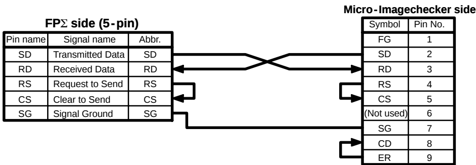
Figure 182: FPΣ Connection example with micro-imagechecker 1
