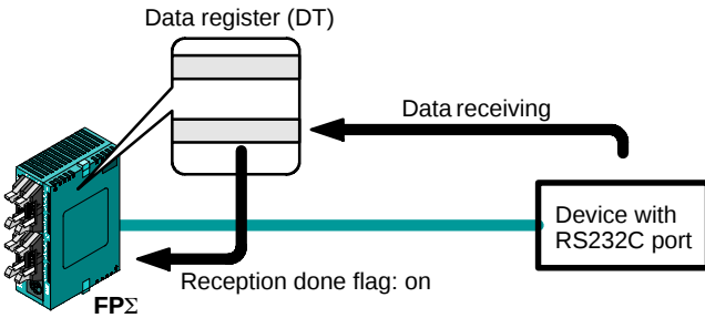
Figure 175: FPΣ Data reception
