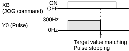
Pulse output diagram
