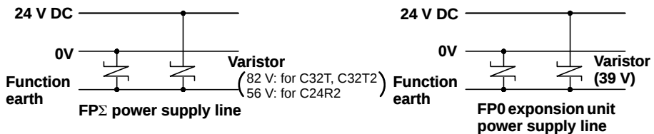
Figure 38: Power supply line of FPΣ and FP0 expansion unit
