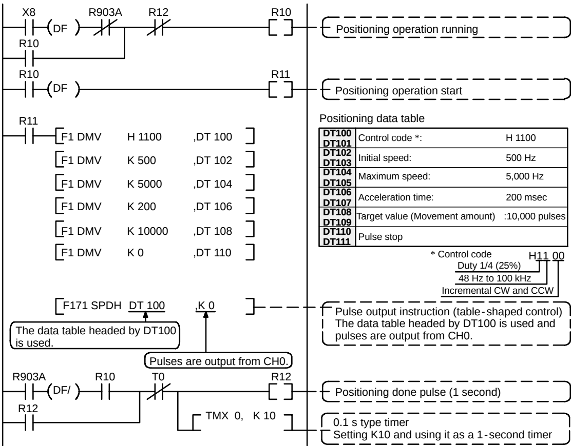
Figure 107: FPΣ Sample program - relative value positioning operation (program)
