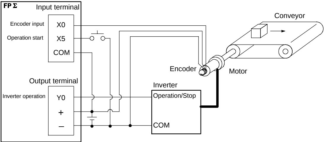
Figure 78: FPΣ High-speed counter function - sample program 1 (wiring)
