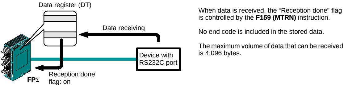
Figure 164: FPΣ Data reception
