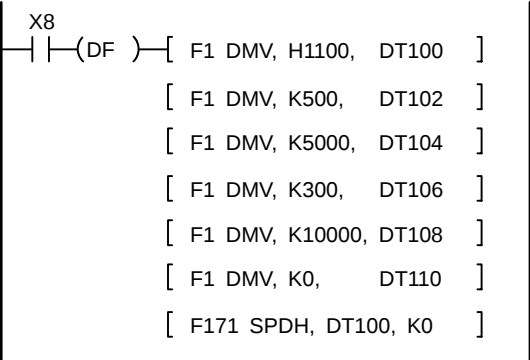
Figure 91: FPΣ Program of positioning control instruction “F171”
