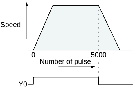
Figure 79: FPΣ High-speed counter function - sample program 1 (operation chart)
