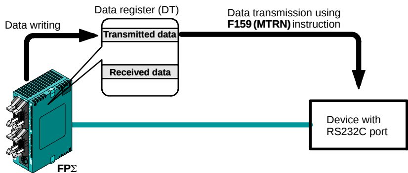
Figure 168: FPΣ Overview of data transmission
