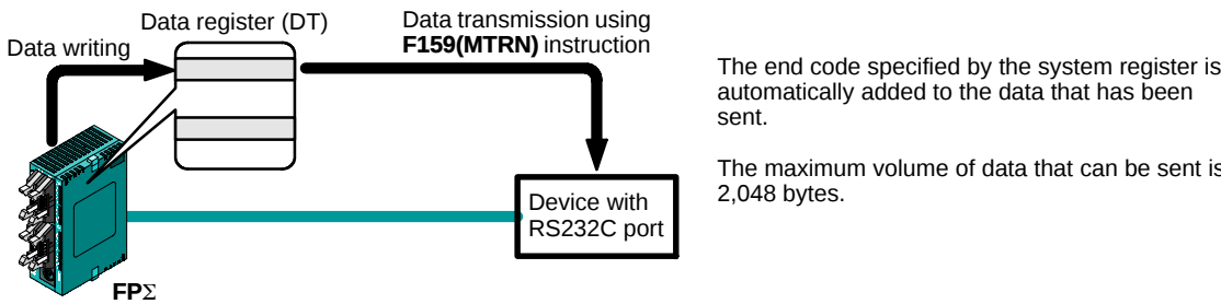
Figure 163: FPΣ Data transmission
