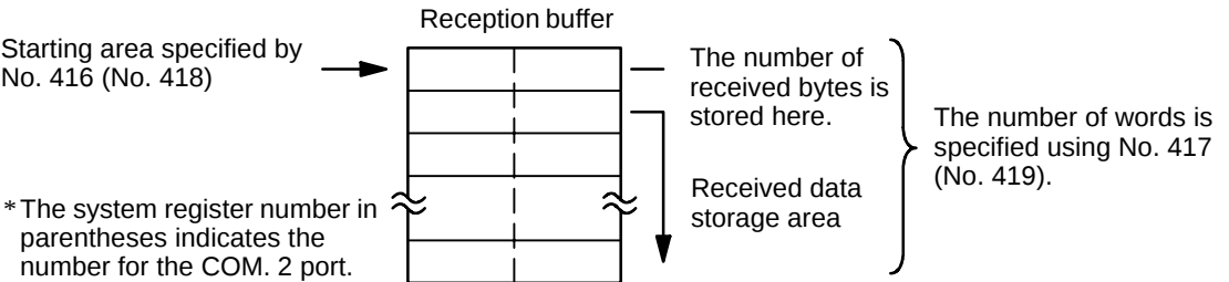
Figure 167: FPΣ Reception buffer
