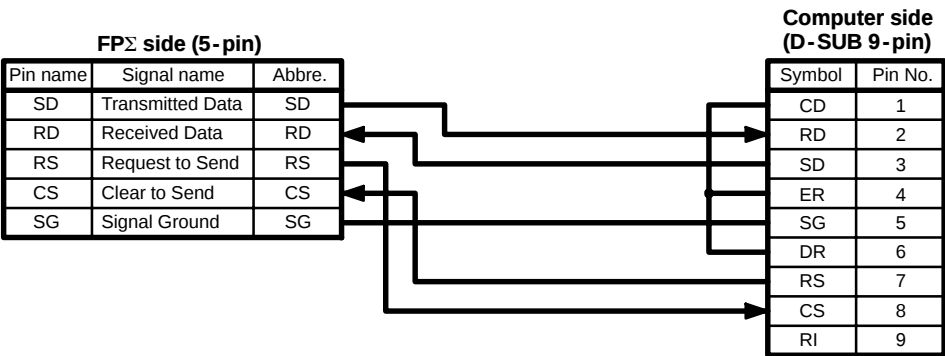
Figure 149: FPΣ Computer link - connection example 1 (computer)
