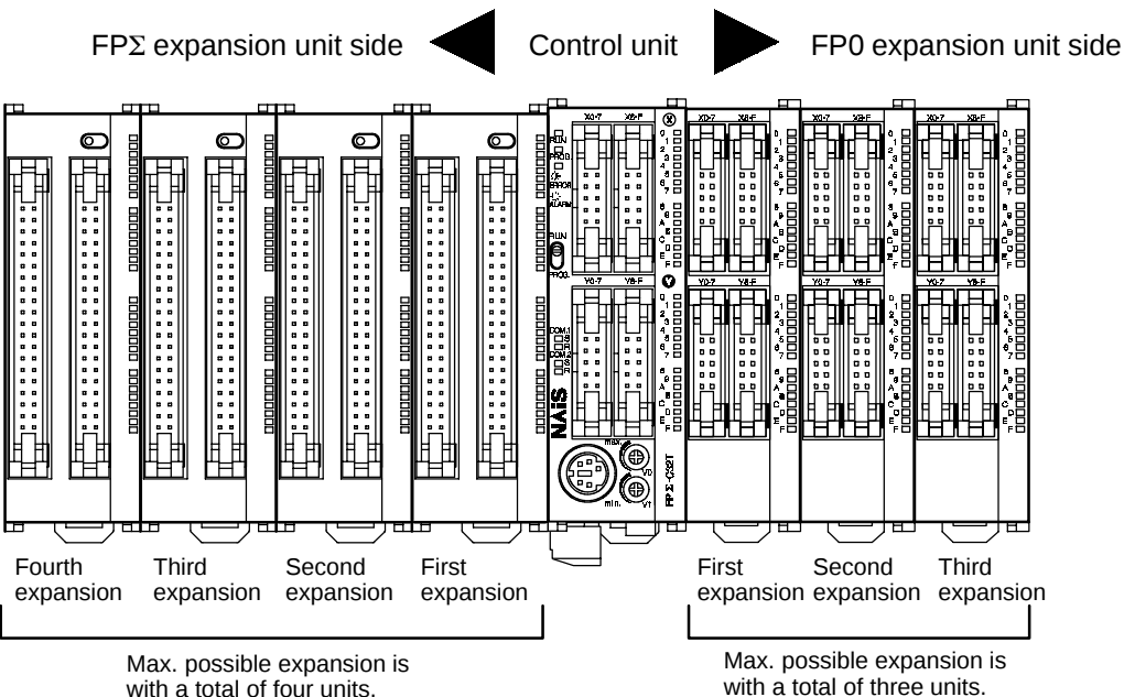
Figure 22: FPΣ I/O allocation
