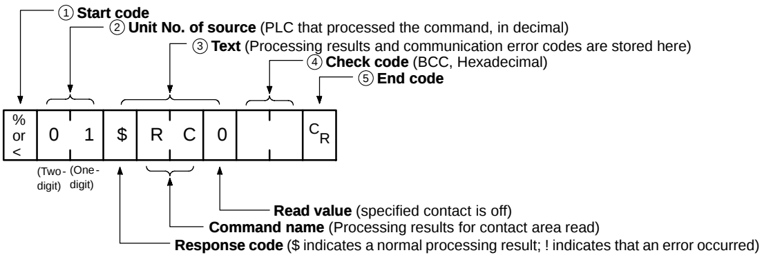
Figure 144: FPΣ Response message (format)
