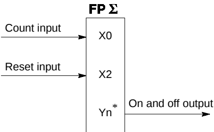
Figure 69: FPΣ High-speed counter function - I/O allocation-1
