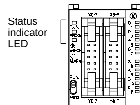
Figure 228: FPΣ Status indicator LED
