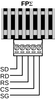
Figure 130: FPΣ 1-channel RS232C type communication cassette
