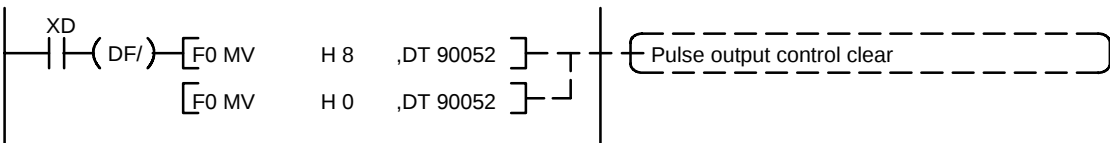
Figure 125: FPΣ Sample program - emergency stop (program)
