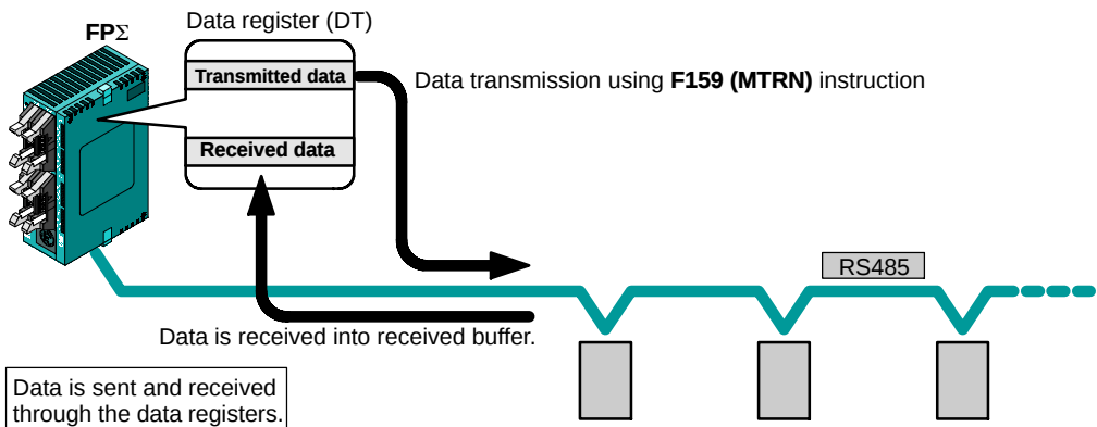
Figure 196: FPΣ General-purpose serial communication (1:N communication)
