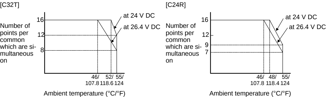
Figure 11: FPΣ Limitations on number of simultaneous input on points
