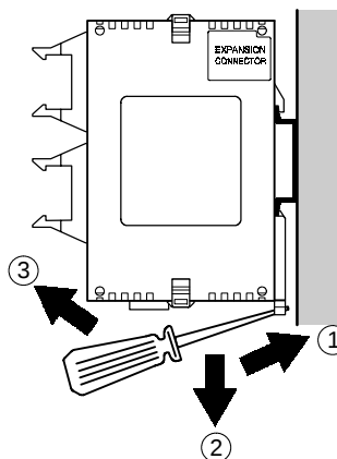
Figure 28: Removal method
