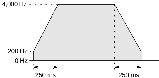
Figure 114: FPΣ Sample program - pulse output diagram
