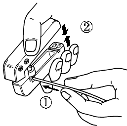
Figure 50: FPΣ MIL connector assembly procedure-2
