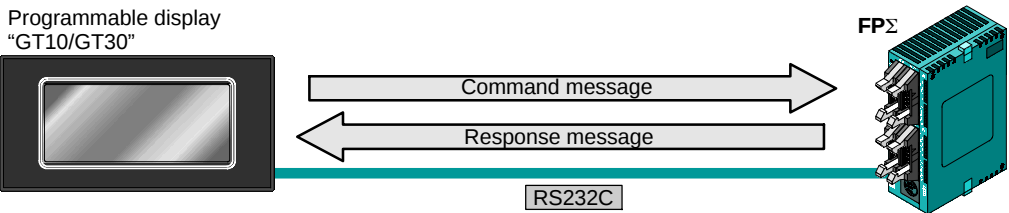
Figure 151: FPΣ Computer link - connection example (GT10)
