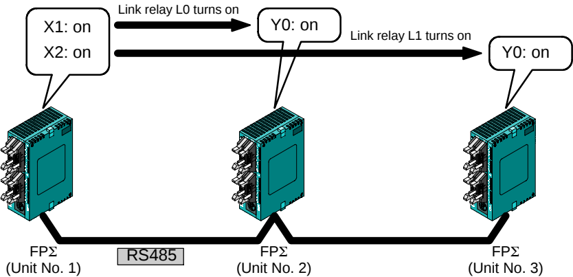
Figure 216: FPΣ Connection when using a PLC link with three FPΣ units
