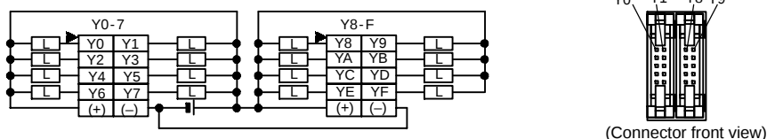
Figure 17: FPΣ Terminal layout diagram (I/O connector)
