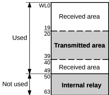
Figure 211: Using only a part of the link relay area
