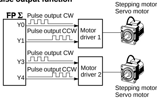
Figure 59: FPΣ Pulse output function
