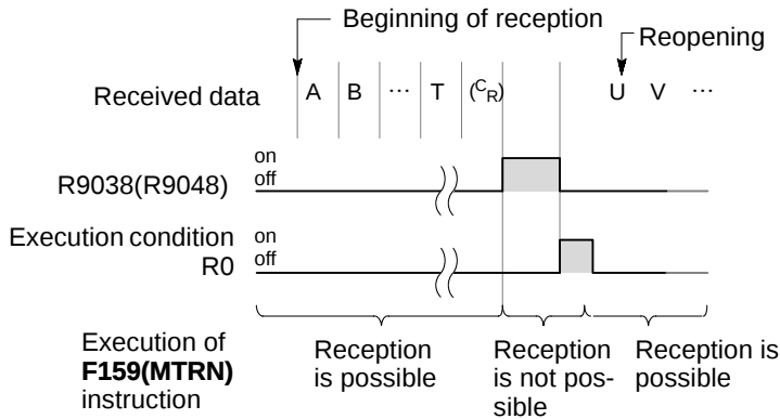
Figure 180: Explanation during reception
