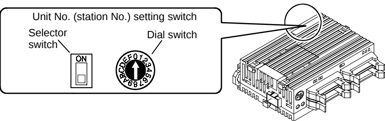
Figure 158: FPΣ Computer link - unit No. (station No.) setting switch
