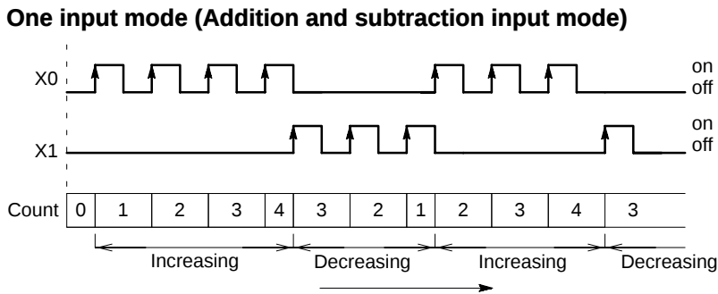
Figure 65: FPΣ High-speed counter function - One input mode
