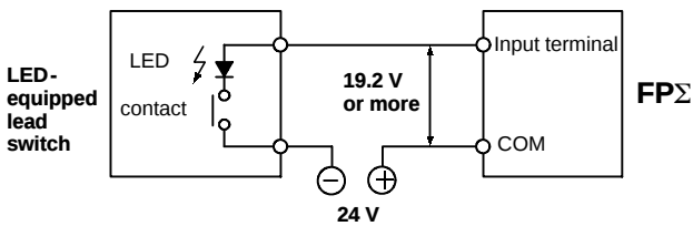
Figure 43: FPΣ Precaution when using LED-equipped lead switch
