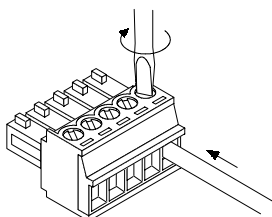
Figure 138: FPΣ Communication connector wiring method 2
