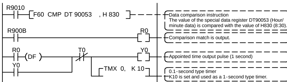
Figure 227: FPΣ Sample program of clock/calendar function
