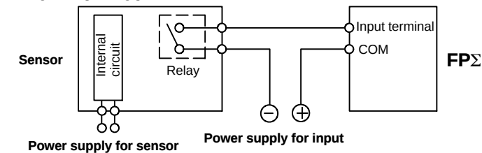
Figure 39: FPΣ Relay output type sensor
