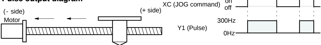
Figure 124: FPΣ Sample program - JOG operation (pulse output diagram)
