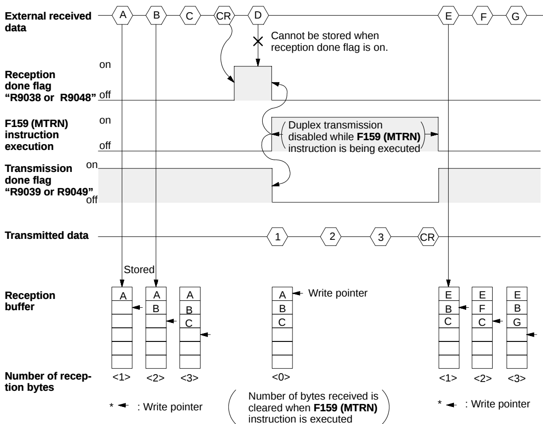
Figure 197: FPΣ Flag operation when receiving data (STX not exit and CR setting)
