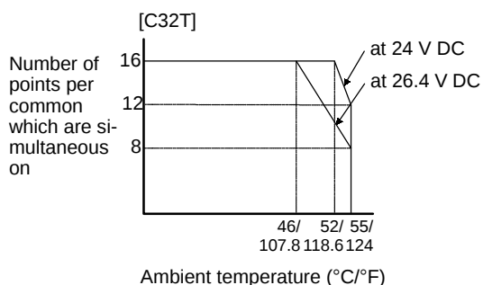
Figure 14: FPΣ Limitations on number of simultaneous output on points
