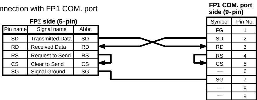
Figure 188: FPΣ Connection example with FP series PLC-1
