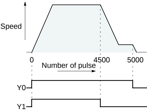
Figure 82: FPΣ High-speed counter function - sample program 2 (operation chart)
