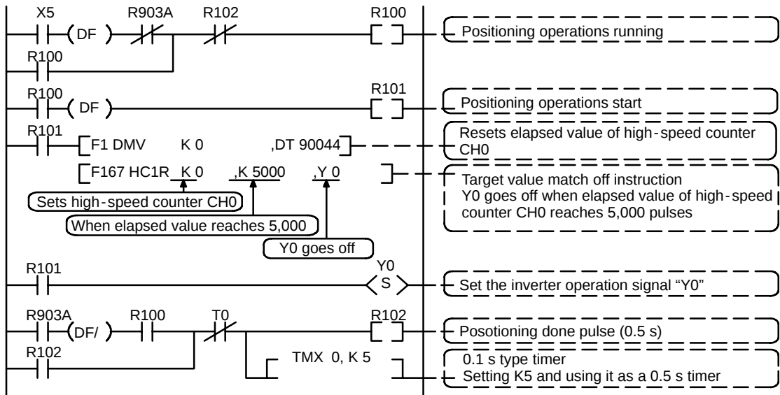
Figure 80: FPΣ High-speed counter function - sample program 1 (program)
