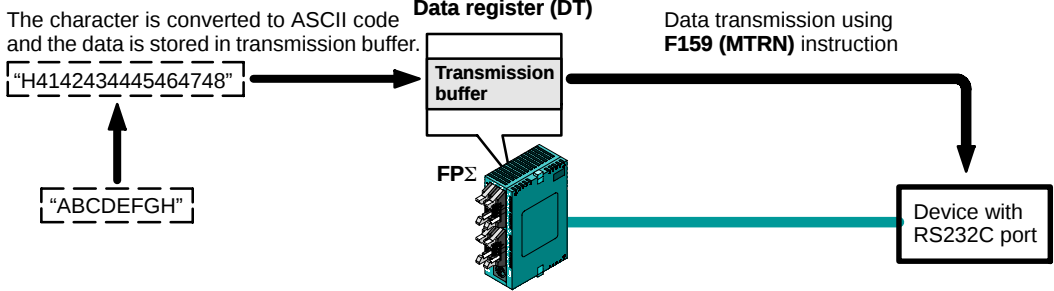
Figure 171: FPΣ Data transmission explanatory diagram
