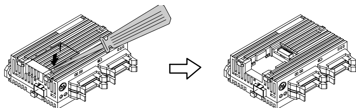
Figure 133: FPΣ Communication cassette attachment procedure 1
