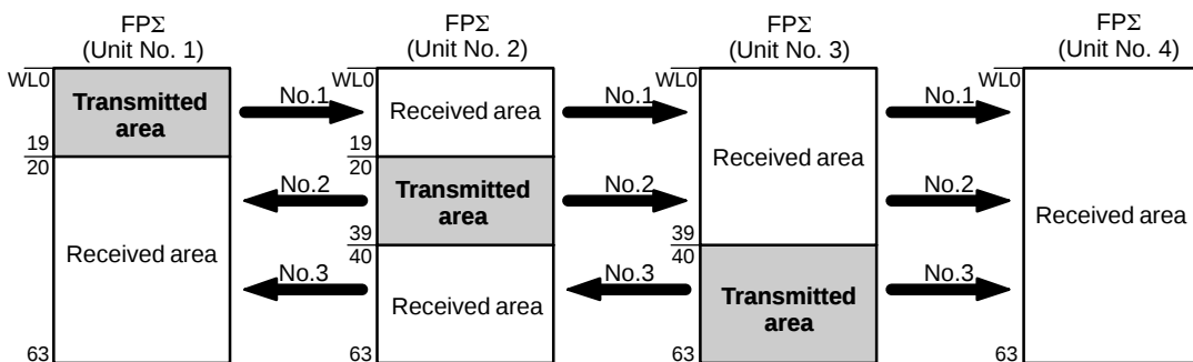
Figure 209: Example of link area allocation
