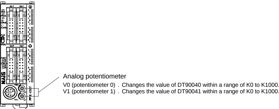
Figure 223: FPΣ Analog potentiometer
