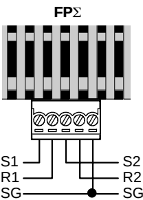
Figure 131: FPΣ 2-channel RS232C type communication cassette
