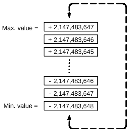
Figure 61: Counting range of high-speed counter
