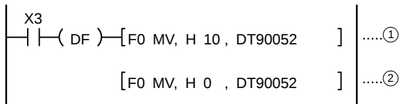
Figure 101: FPΣ Program 1 of pulse output control instruction "F0"
