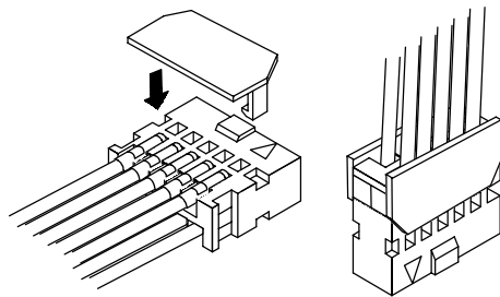
Figure 52: FPΣ MIL connector assembly procedure-4
