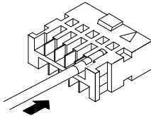
Figure 51: FPΣ MIL connector assembly procedure-3
