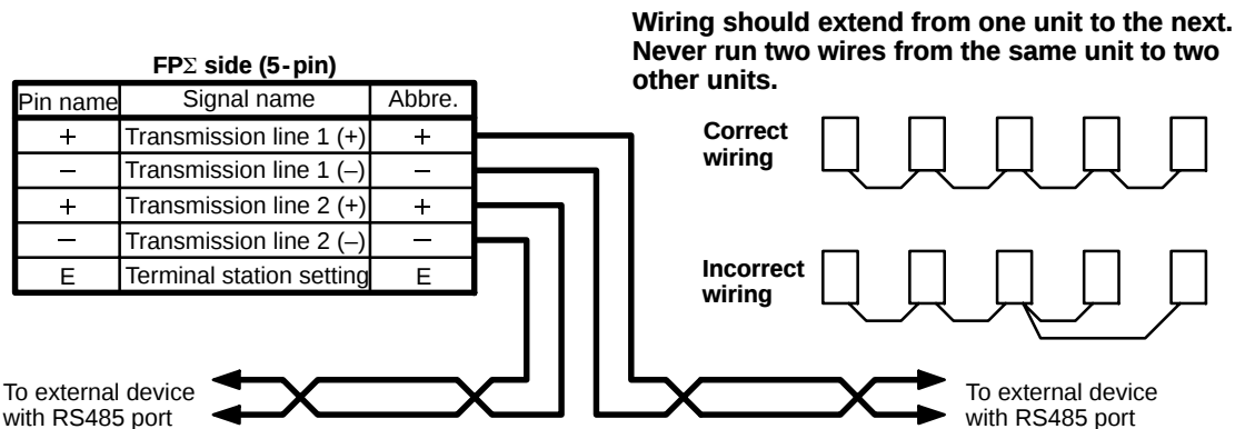
Figure 160: FPΣ Computer link - connection diagram
