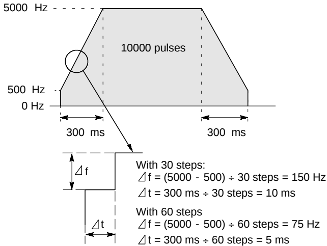
Figure 92: FPΣ Pulse output diagram of "F171" instruction
