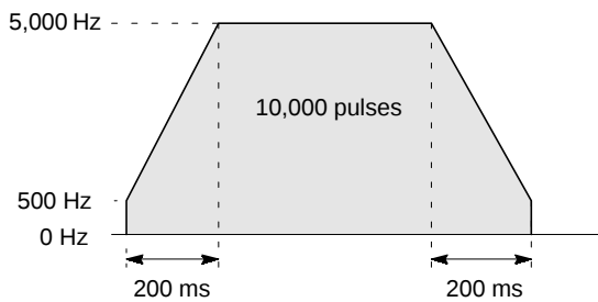
Figure 108: FPΣ Sample program - pulse output diagram
