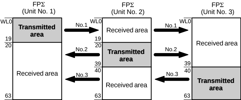
Figure 217: FPΣ Link relay allocation when using a PLC link with three FPΣ units
