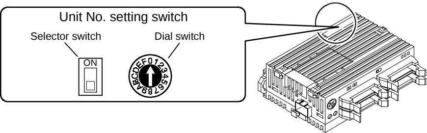
Figure 206: FPΣ Unit No. setting switch
