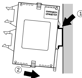
Figure 27: Installation method
