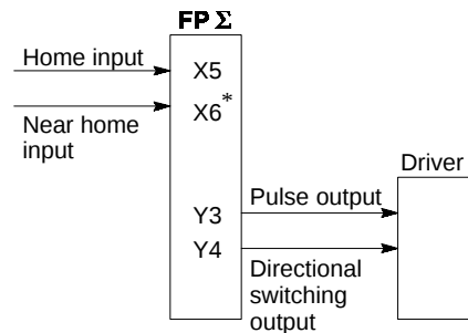
Figure 90: FPΣ Pulse output function - I/O allocation when using CH2 (single pulse input)
