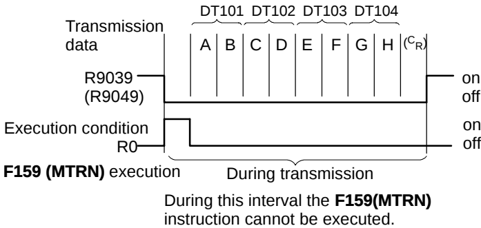
Figure 173: Explanation during transmission
