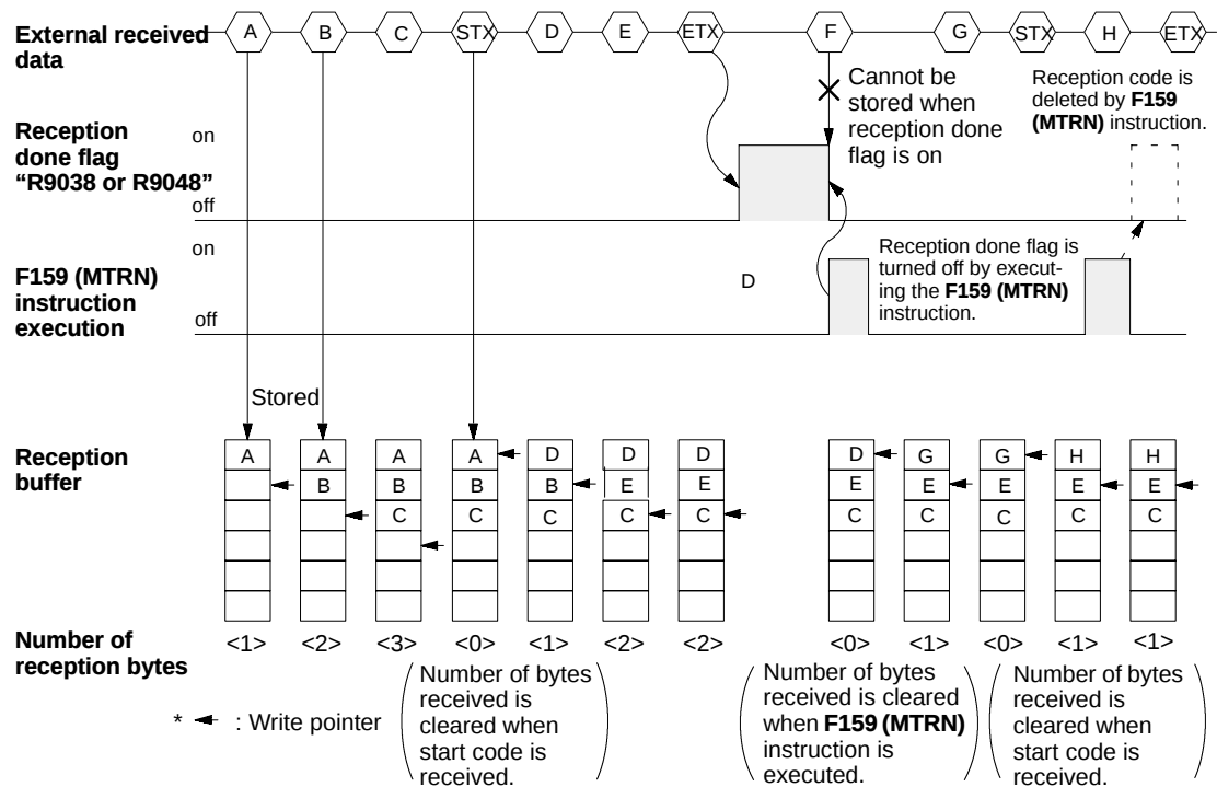
Figure 198: FPΣ Flag operation when receiving data (STX and ETX setting)
