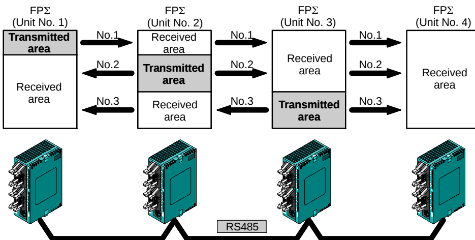
Figure 201: FPΣ PLC link function (overview)
