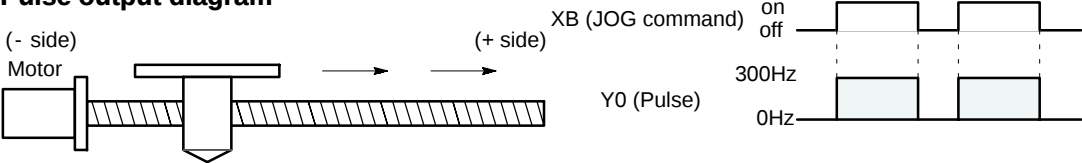
Figure 122: FPΣ Sample program - JOG operation (pulse output diagram)
