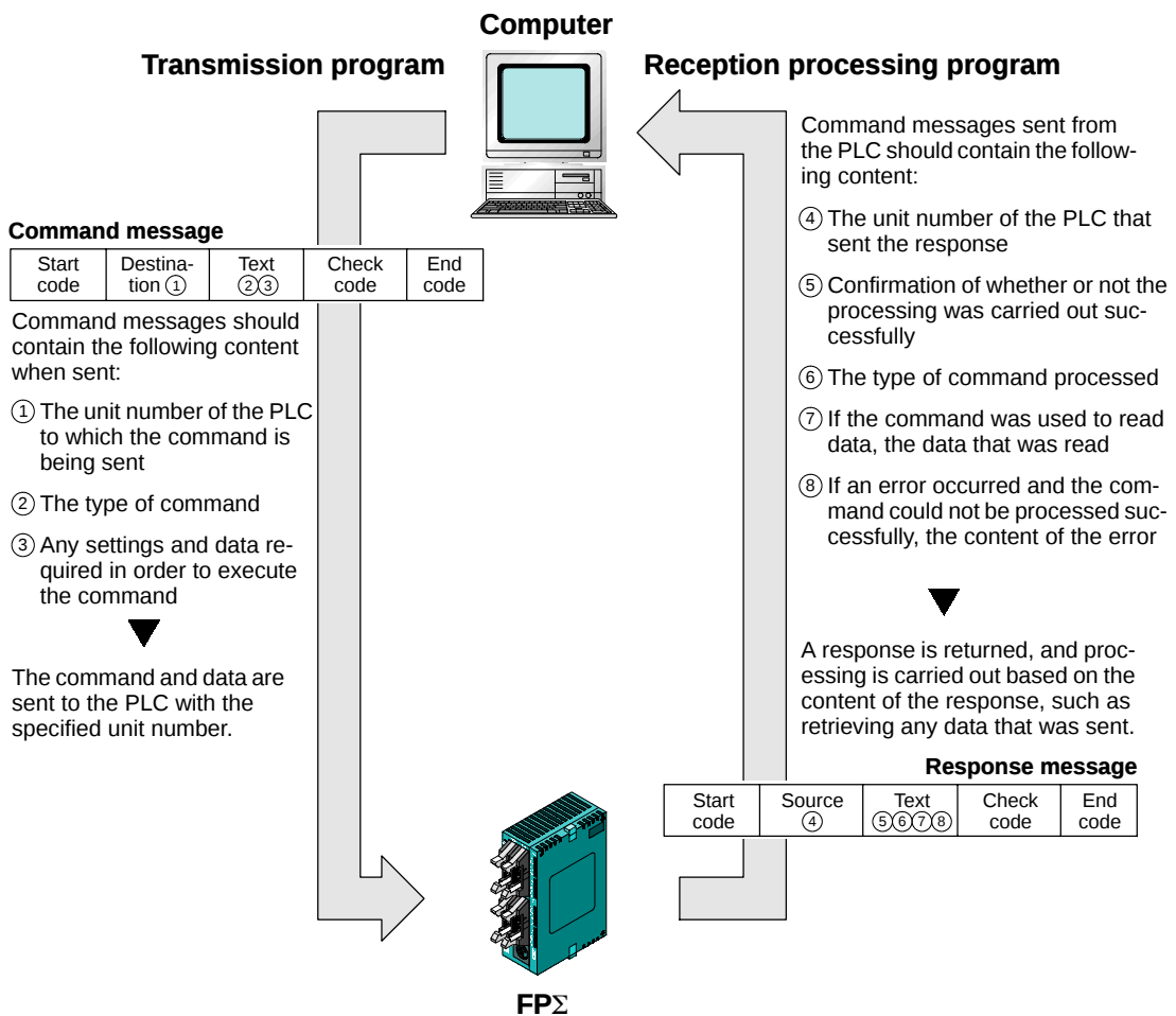
Figure 141: FPΣ MEWTOCOL - COM
