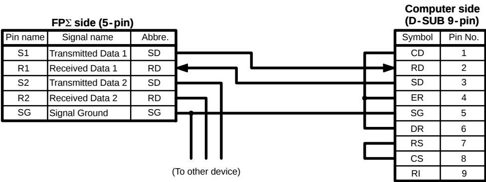
Figure 150: FPΣ Computer link - connection example 2 (computer)
