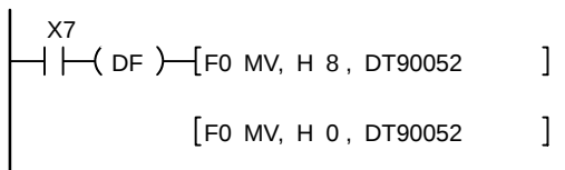
Figure 102: FPΣ Program 2 of pulse output control instruction "F0"
