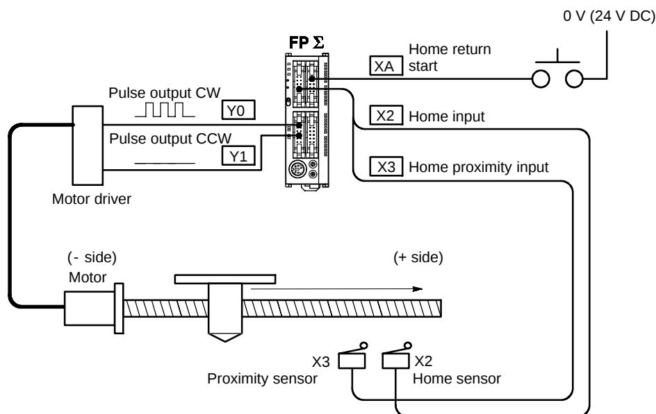
Figure 118: FPΣ Sample program - home return operation (+ direction)
