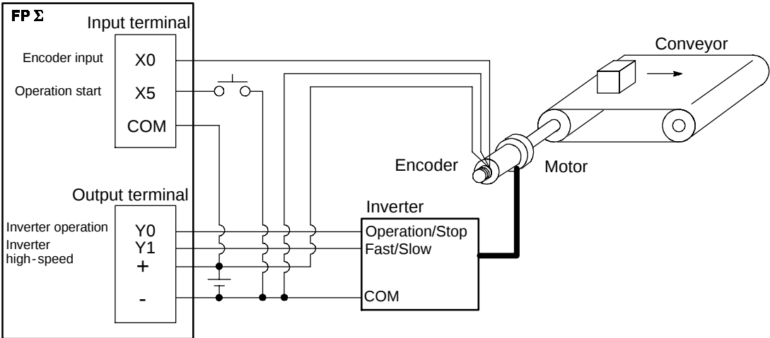
Figure 81: FPΣ High-speed counter function - sample program 2 (wiring)
