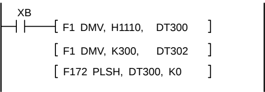
Figure 98: FPΣ Program of pulse output instruction “F172”
