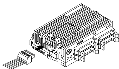
Figure 135: FPΣ Communication cassette attachment procedure 3
