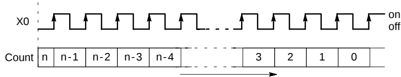
Figure 63: FPΣ High-speed counter function - subtraction input mode
