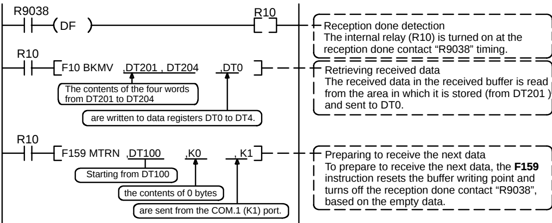
Figure 176: FPΣ Sample program for data reception
