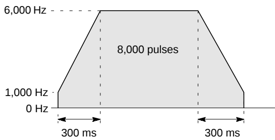
Figure 111: FPΣ Sample program - pulse output diagram
