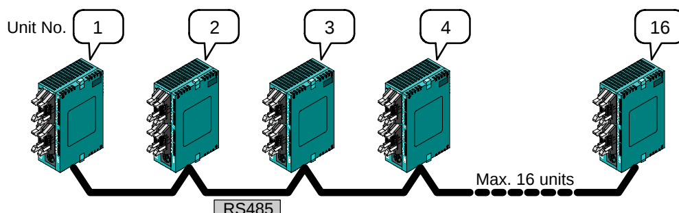
Figure 204: FPΣ Unit No. for PLC link
