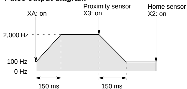
Figure 117: FP\Sigma Sample program - home return operation (pulse output diagram)
