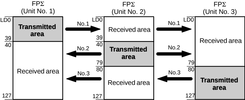
Figure 218: FPΣ Link register allocation when using a PLC link with three FPΣ units
