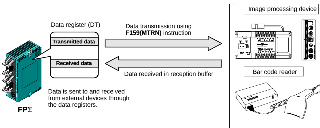
Figure 128: FPΣ General-purpose serial communication function
