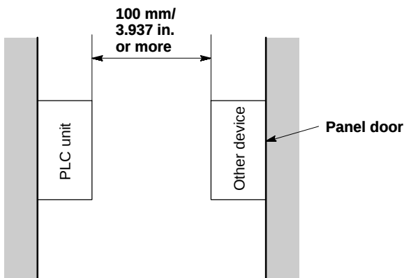
Figure 26: FPΣ Installation space -2
