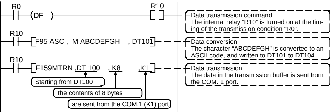
Figure 170: FPΣ Sample program for data transmission
