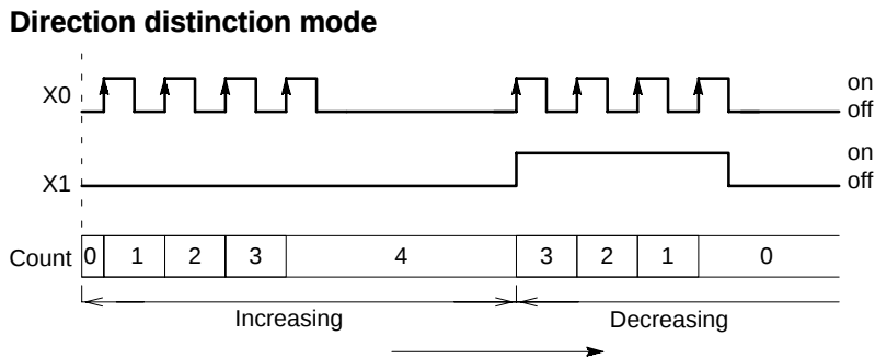
Figure 66: FPΣ High-speed counter function - direction distinction mode
