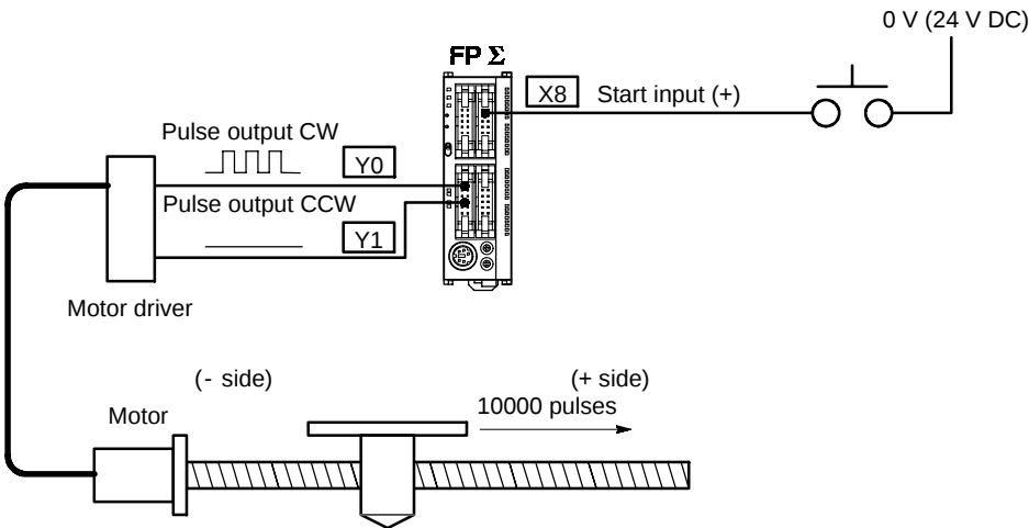
Figure 106: FPΣ Sample program - relative value positioning operation (+ direction)
