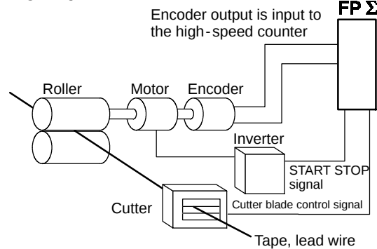
Figure 58: FPΣ High-speed counter function
