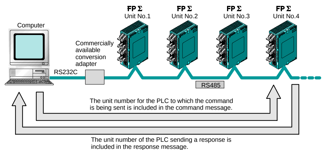
Figure 156: FPΣ Overview of compute link function (1:N communication)
