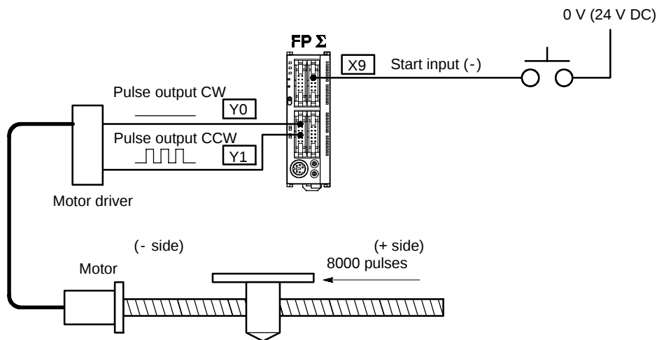
Figure 109: FPΣ Sample program - relative value positioning operation (– direction)
