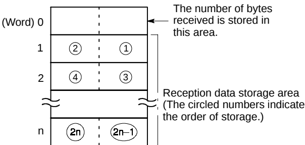
Figure 179: FPΣ Data table for reception
