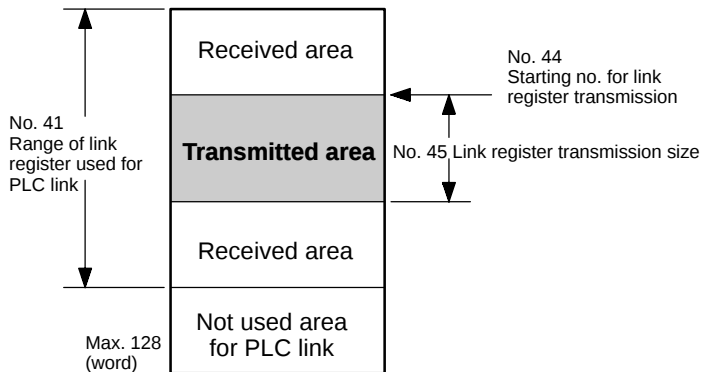
Figure 208: FPΣ Link register allocation
