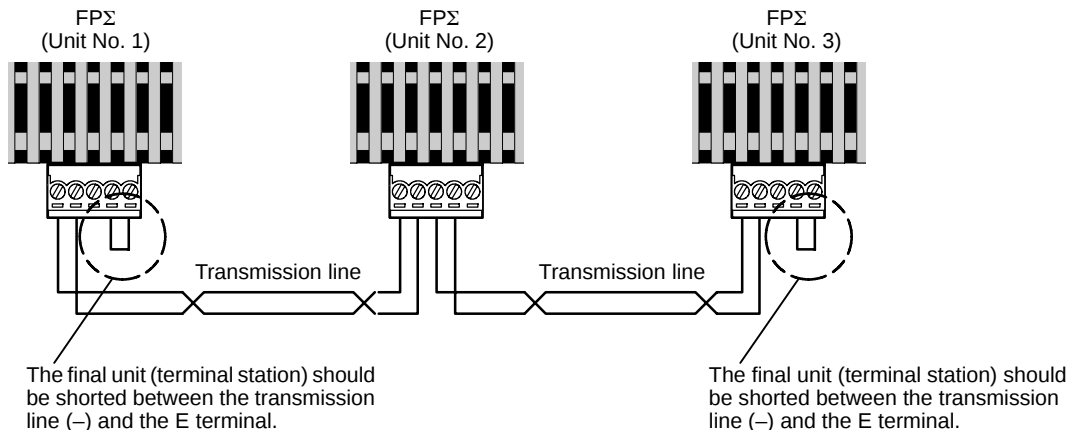
Figure 219: FPΣ Connection diagram when using a PLC link with three FPΣ units
