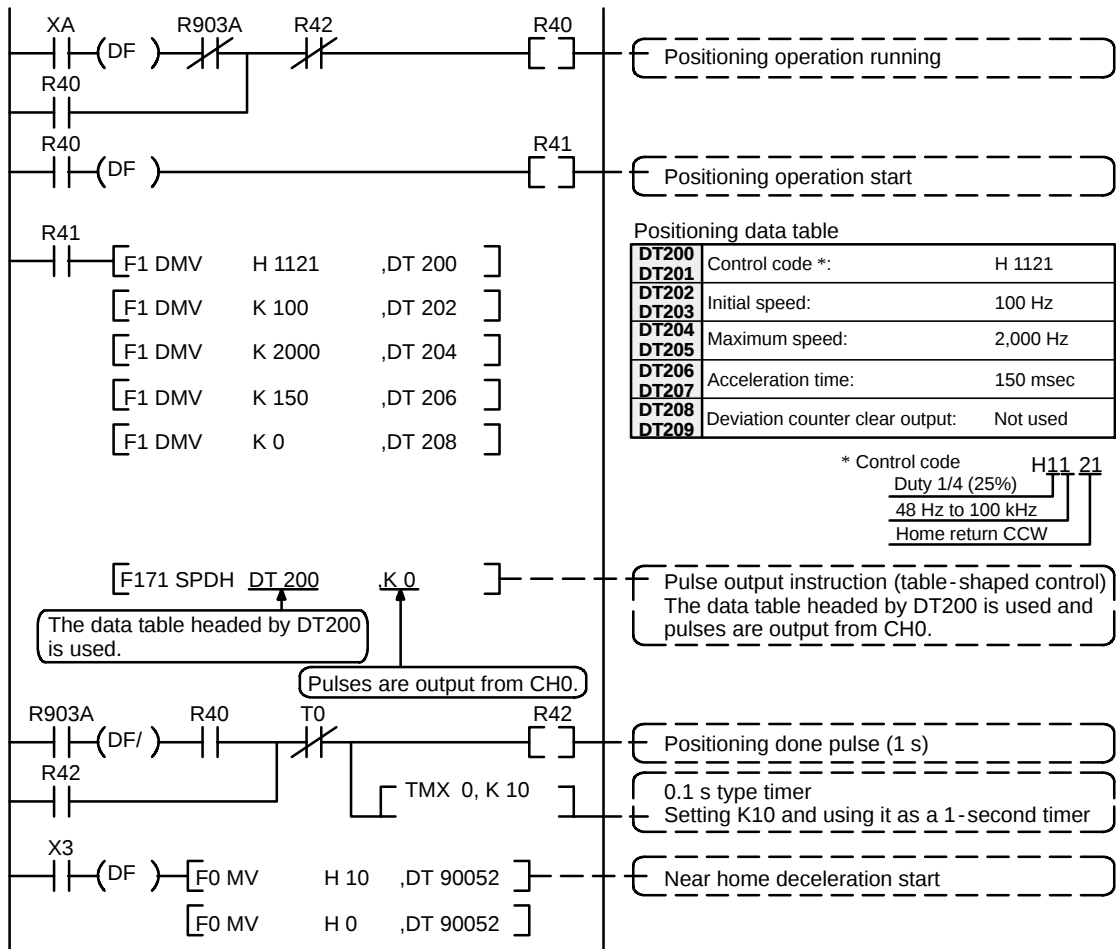
Figure 116: FP\Sigma Sample program - home return operation (program)
