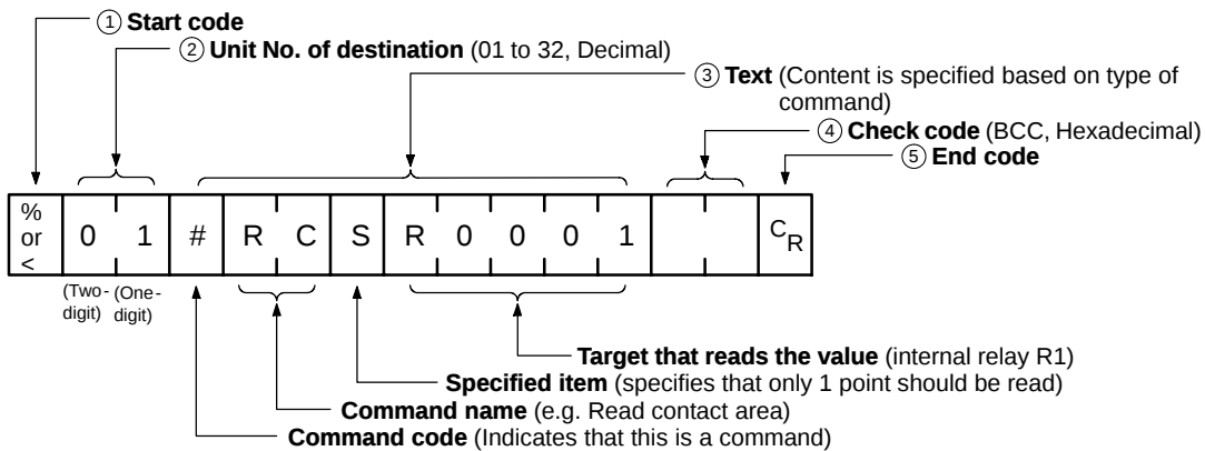
Figure 142: FPΣ Command message (format)
