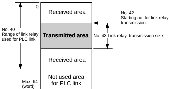
Figure 207: FPΣ Link relay allocation
