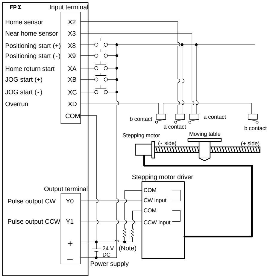
Figure 105: FPΣ Pulse output function - sample program (wiring)
