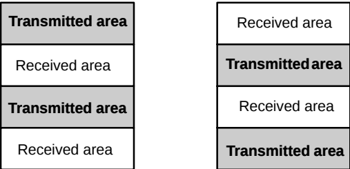
Figure 215: Unallowable allocation example 2
