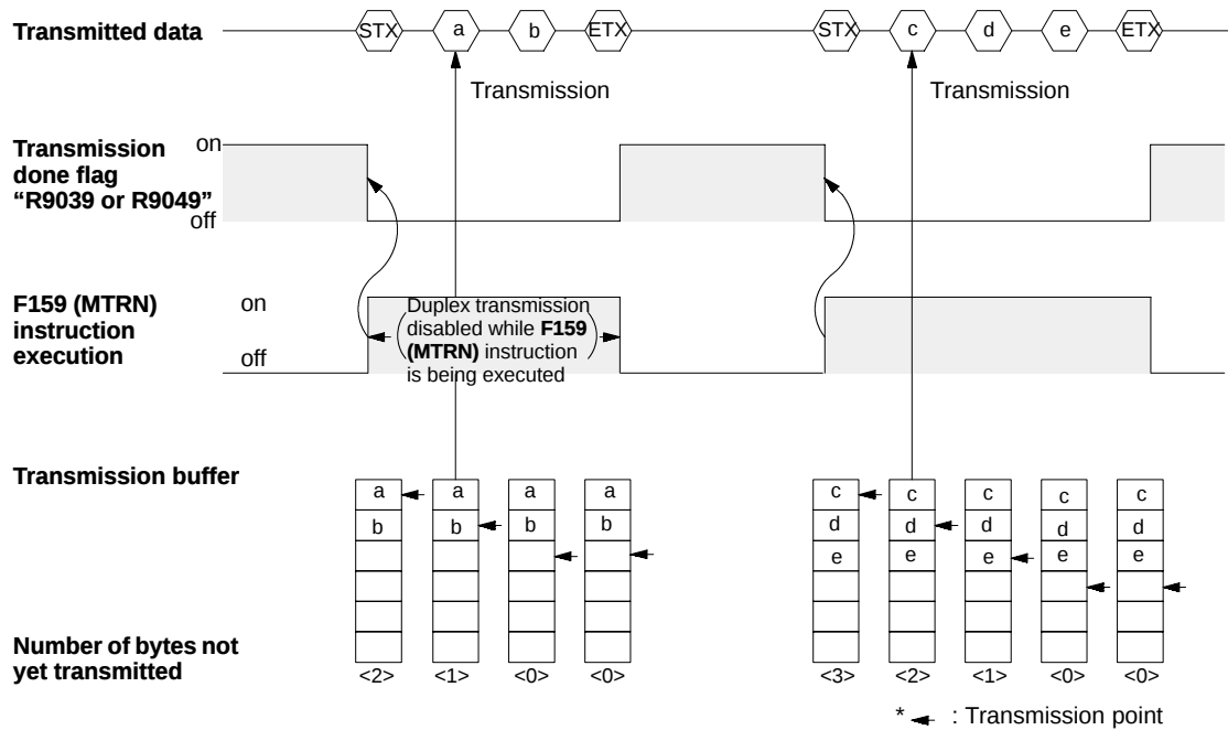
Figure 199: FPΣ Flag operation when sending data (STX and ETX setting)
