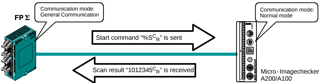
Figure 181: FPΣ Connection example with external device (micro-imagechecker)
