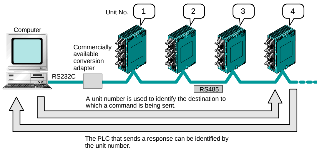
Figure 157: FPΣ Computer link - setting of unit No. (station No.)
