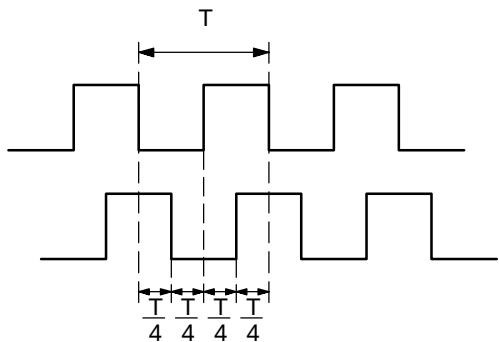
Figure 68: FPΣ High-speed counter function - min. input pulse width (two-phase)
