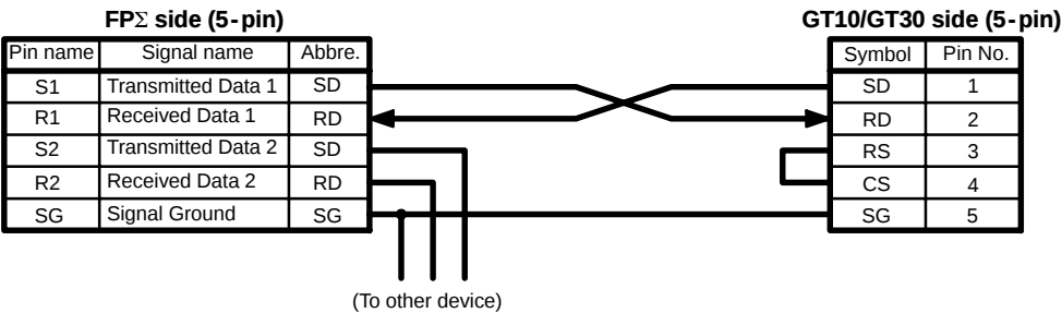
Figure 154: FPΣ Computer link - connection example 2 (GT10)
