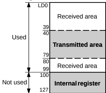
Figure 212: Using only a part of the link register area
