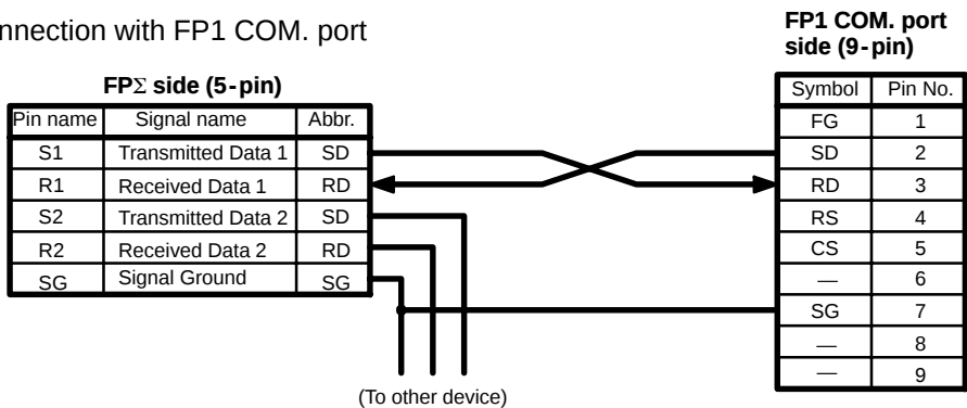
Figure 189: FPΣ Connection example with FP series PLC-2
