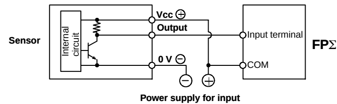
Figure 41: FPΣ Voltage output (universal output) type sensor
