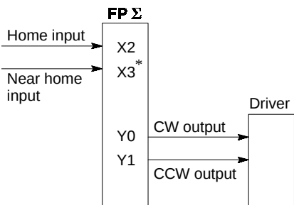
Figure 87: FPΣ Pulse output function - I/O allocation when using CH0 (double pulse input)
