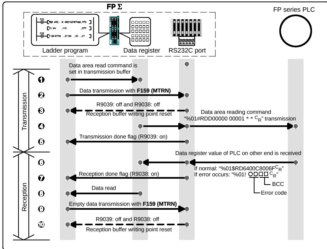
Figure 190: FPΣ Procedure of communication (FP series PLC)
