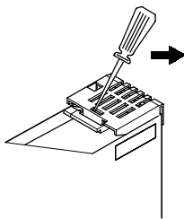
Figure 54: FPΣ Backup battery installation procedure-1
