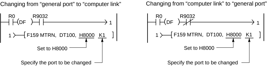
Figure 200: FPΣ Changing the communication mode of COM. port
