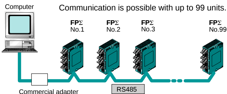
Figure 2: Features-communication (C-NET)
