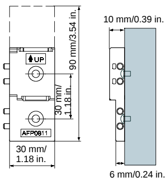
Figure 29: FPΣ Installation -optional slim 30 type mounting plate
