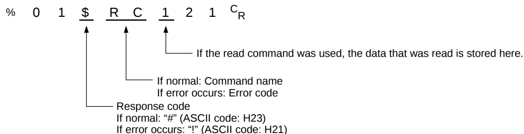
Figure 145: FPΣ Response message (text)
