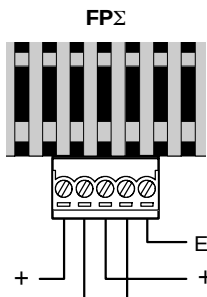
Figure 132: FPΣ 1-channel RS485 type communication cassette
