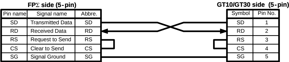
Figure 153: FPΣ Computer link - connection example 1 (GT10)
