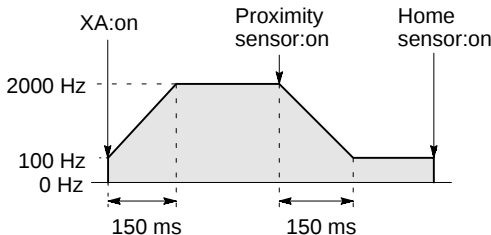
Figure 95: FPΣ Pulse output diagram of “F171” instruction
