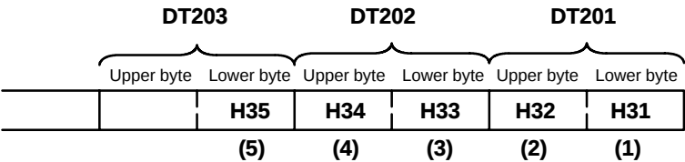
Figure 195: FPΣ Example (received buffer)
