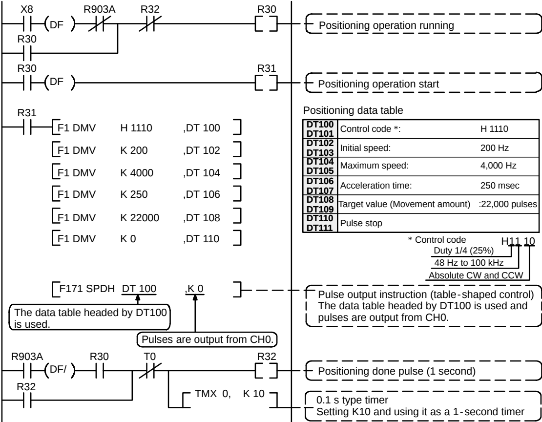
Figure 113: FPΣ Sample program - absolute value positioning operation (program)
