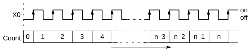
Figure 62: FPΣ High-speed counter function - addition input mode
