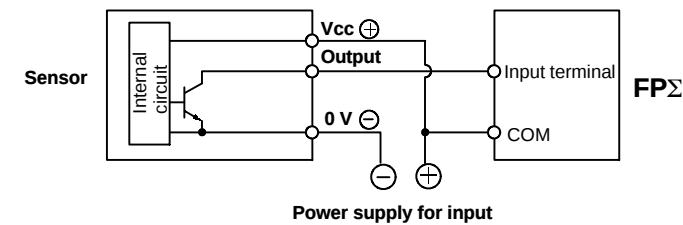
Figure 40: FPΣ NPN open collector output type sensor
