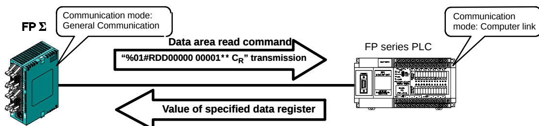
Figure 187: FPΣ Connection example with external device (FP series PLC)
