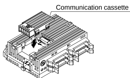
Figure 134: FPΣ Communication cassette attachment procedure 2
