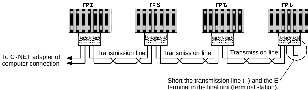
Figure 161: FPΣ Computer link - terminal station setting
