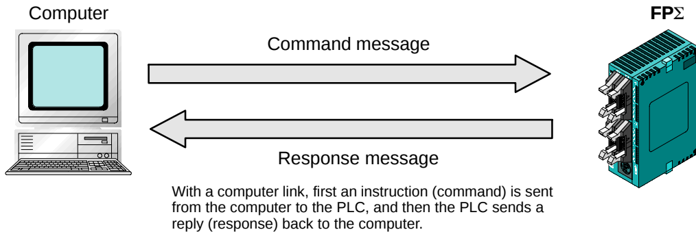
Figure 140: FPΣ Overview of computer link function
