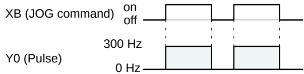
Figure 99: FPΣ Pulse output diagram of “F172” instruction
