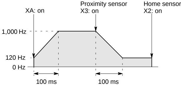
Figure 120: FPΣ Sample program - home return operation (pulse output diagram)
