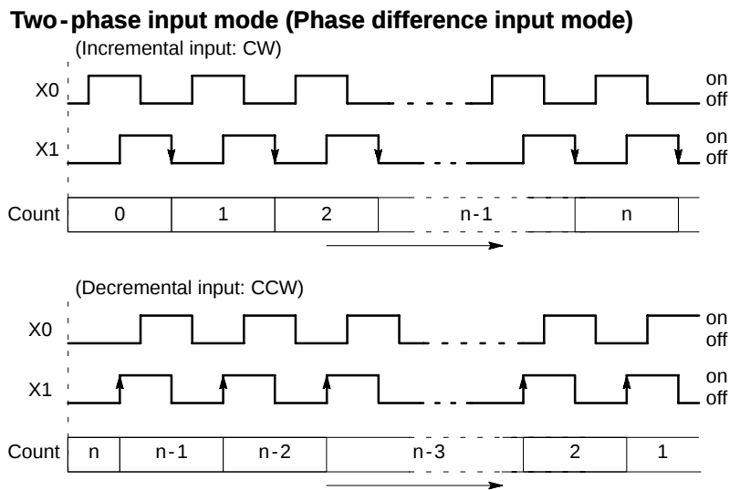
Figure 64: FPΣ High-speed counter function - two-phase input mode
