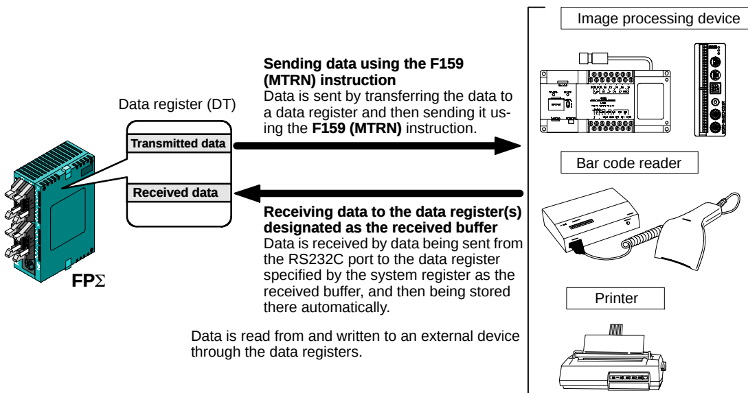
Figure 162: FPΣ General-purpose Serial Communication (overview)
