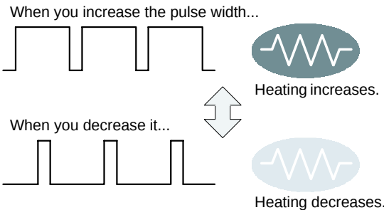
Figure 60: FPΣ PWM output function
