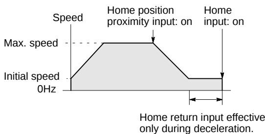
Figure 97: FPΣ Home return operation modes
