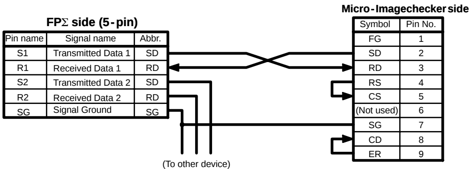
Figure 183: FPΣ Connection example with micro-imagechecker 2
