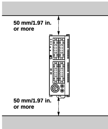
Figure 25: FPΣ Installation space -1
