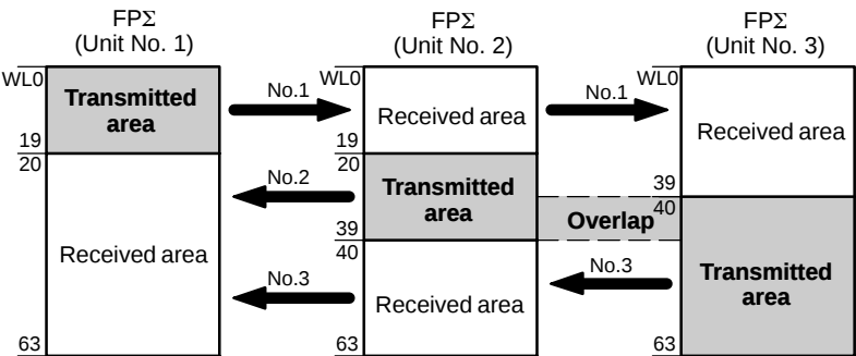
Figure 213: Precautions when allocating link relay area
