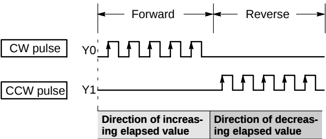
Figure 84: FPΣ Pulse output function - CW/CCW output method
