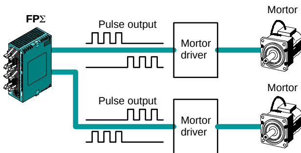
Figure 5: Features-Pulse output
