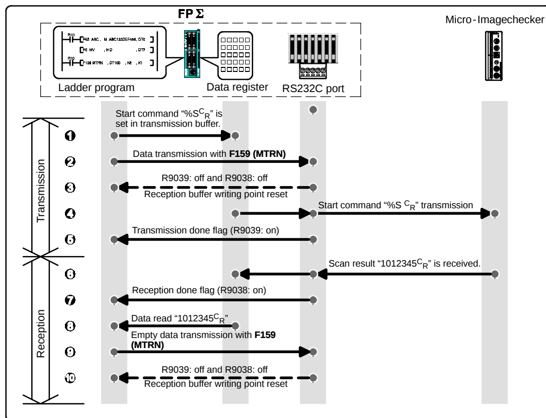
Figure 184: FPΣ Procedure of communication (micro-imagechecker)
