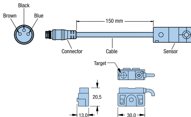
Sensor / Bracket Detail
