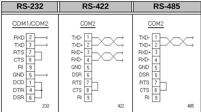
Figure 3-3Pinouts and Cable Settings
