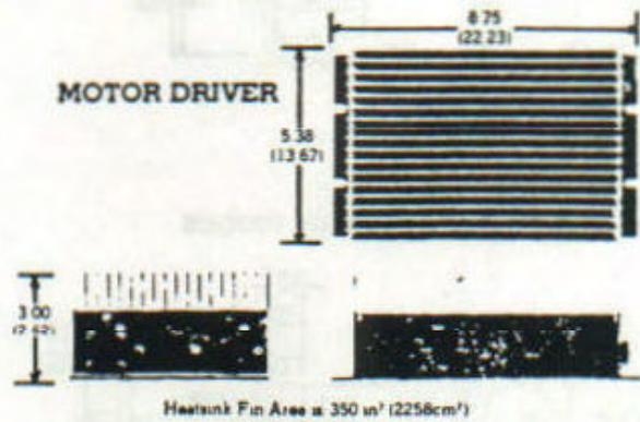
Fig. 6 - Driver Dimensions
