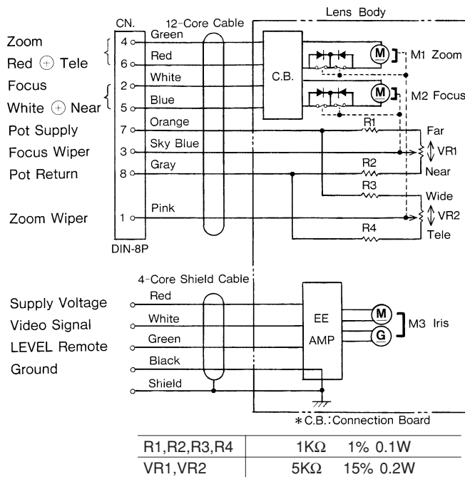
TYPE 1 (DC6V) / TYPE 5 (DC12V)
