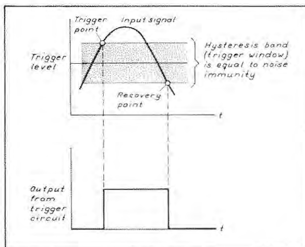
Fig. 7.3 Illustration of the trigger function.
