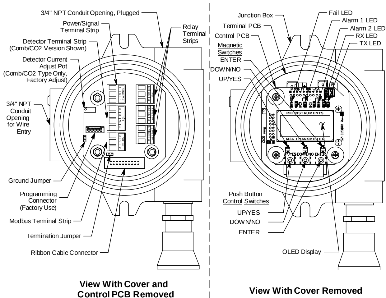
Figure 9: M2A Internal Components
