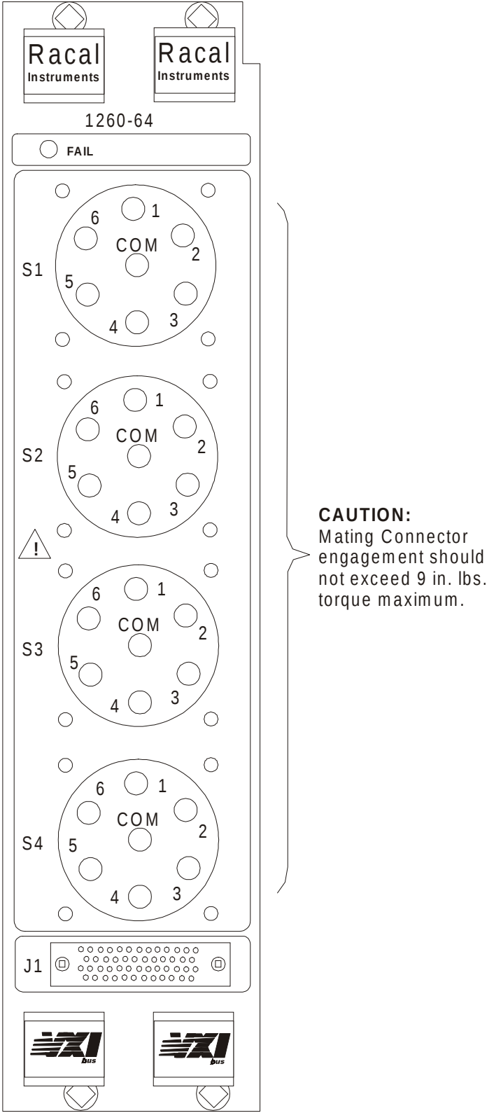
Figure 4-1, 1260-64 Front Panel
